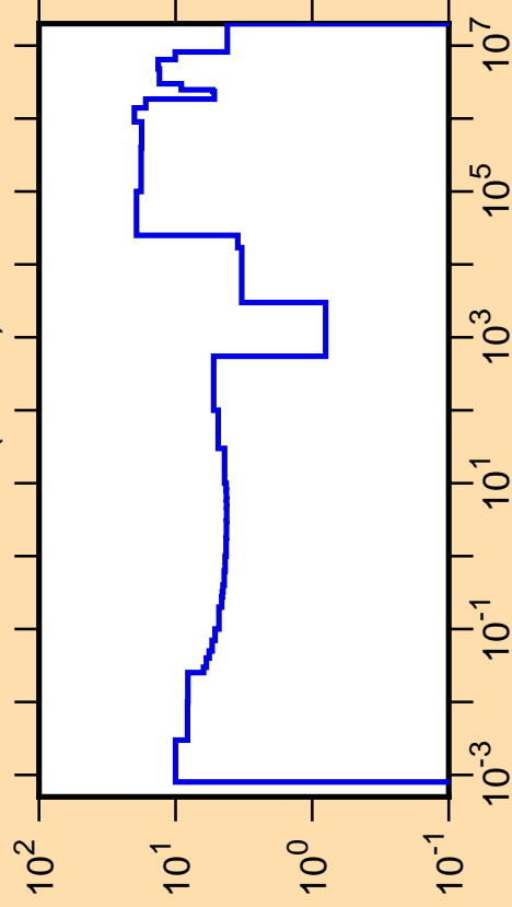
\Delta\sigma/\sigma vs. E for ^{194}\text{W}(n,\text{tot.})
