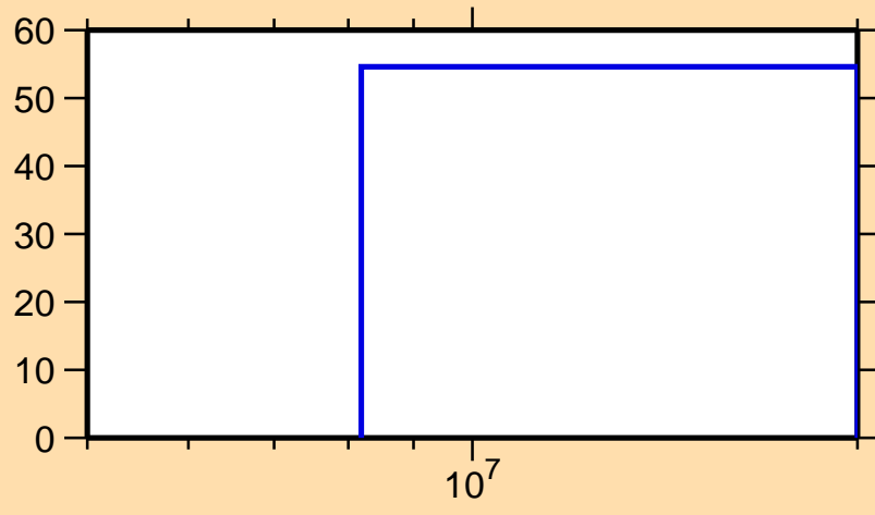
\Delta\sigma/\sigma vs. E for ^{194}\text{W}(n,ncont.)
