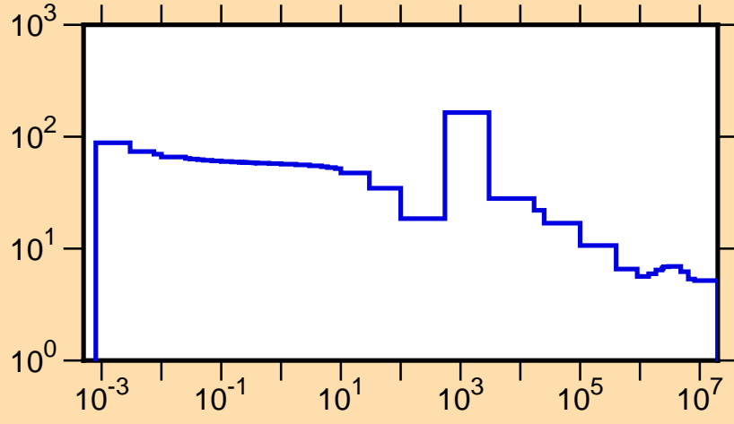
\sigma vs. E for ^{194}\text{W}(n,\text{tot.})
