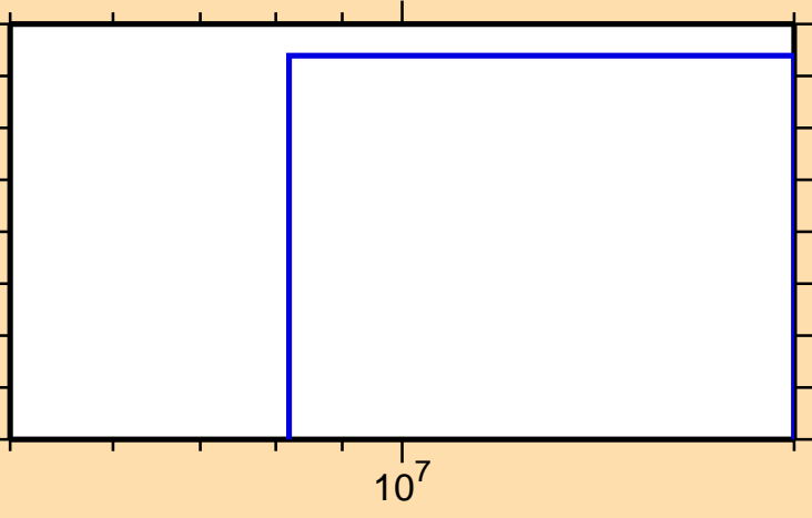
\sigma vs. E for ^{194}\text{W}(n,p)
