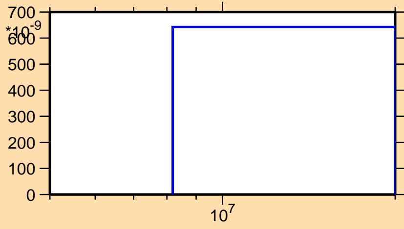
\sigma vs. E for ^{194}\text{W}(n,d)
