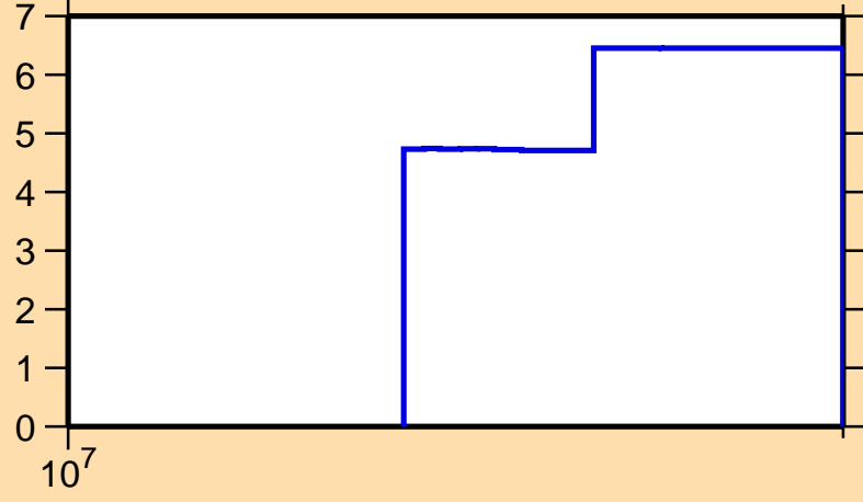
\Delta\sigma/\sigma vs. E for ^{112}\text{Xe}(n,\text{tot.})
