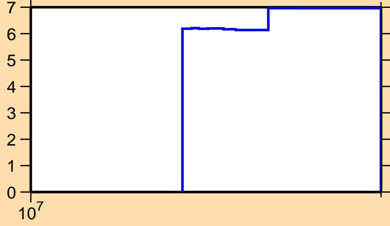
\Delta\sigma/\sigma vs. E for ^{112}\text{Xe}(n,\text{el.})
