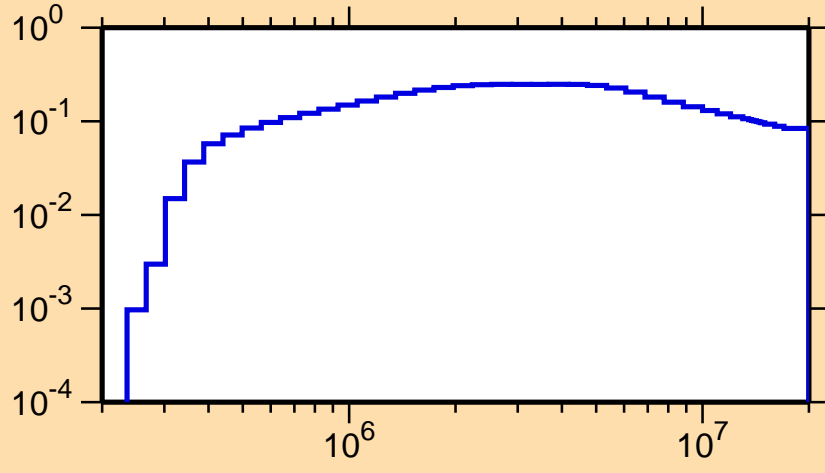
\sigma vs. E for ^{112}\text{Xe}(n,n_1)
