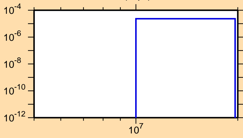
\sigma vs. E for ^{112}\text{Xe}(n,pt)
