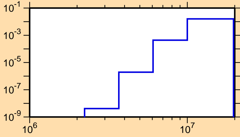
\sigma vs. E for ^{112}\text{Xe}(n,d)
