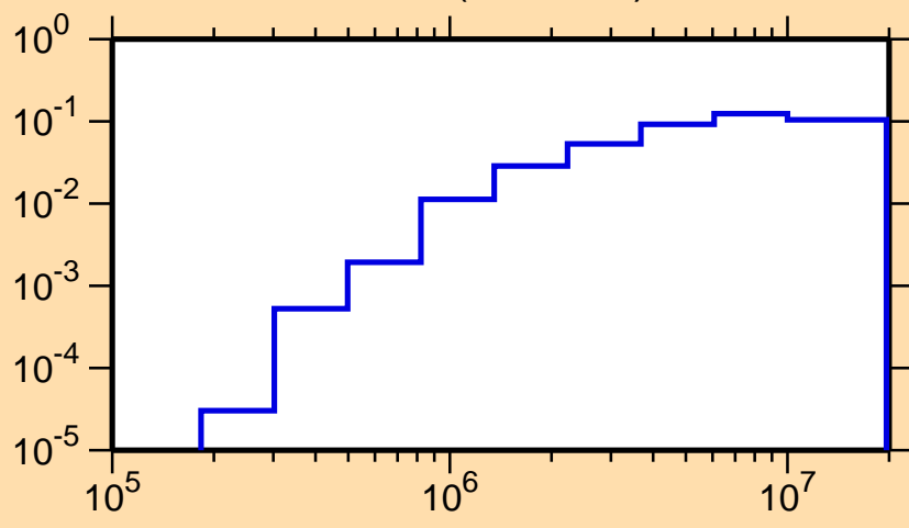
\sigma vs. E for ^{112}\text{Xe}(n,n\text{cont.})
