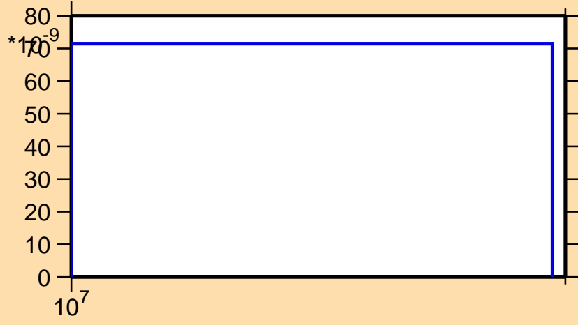
\sigma vs. E for ^{112}\text{Xe}(n,2n\alpha)
