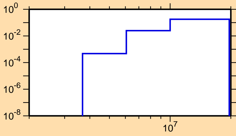
\sigma vs. E for ^{112}\text{Xe}(n,np)
