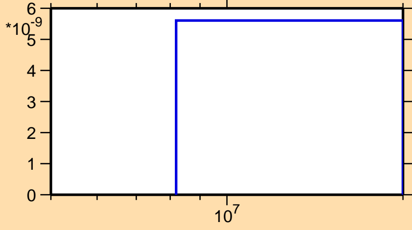
\sigma vs. E for ^{112}\text{Xe}(n,2np)
