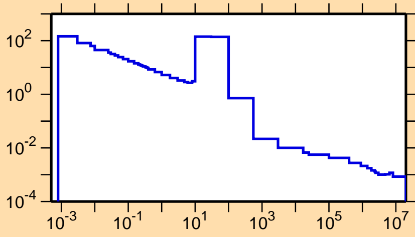
\sigma vs. E for ^{112}\text{Xe}(n,\gamma)
