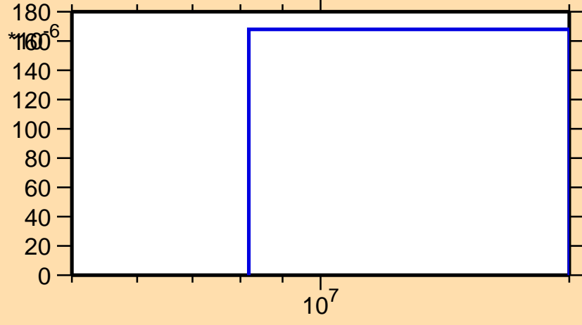
\sigma vs. E for ^{112}\text{Xe}(n,t)
