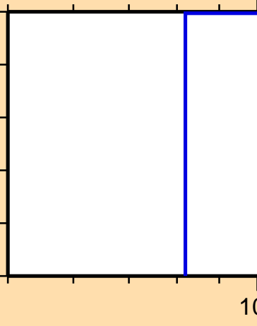
\sigma vs. E for ^{112}\text{Xe}(n,2n)
