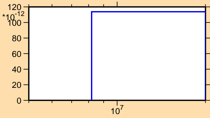
\sigma vs. E for ^{112}\text{Xe}(n,\text{nd})
