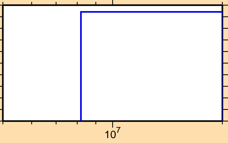
\sigma vs. E for ^{112}\text{Xe}(n,\text{pt})
