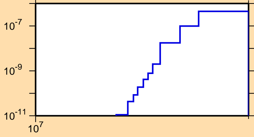
\sigma vs. E for ^{113}\text{Xe}(n,2n\alpha)
