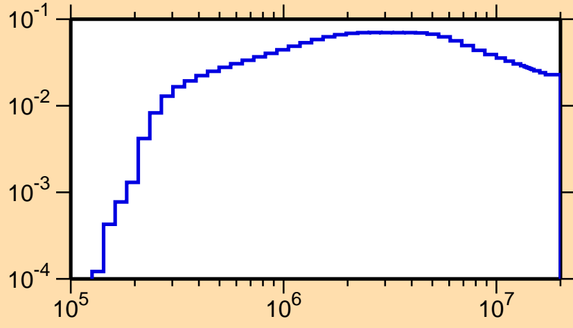
\sigma vs. E for ^{113}\text{Xe}(n,n_1)
