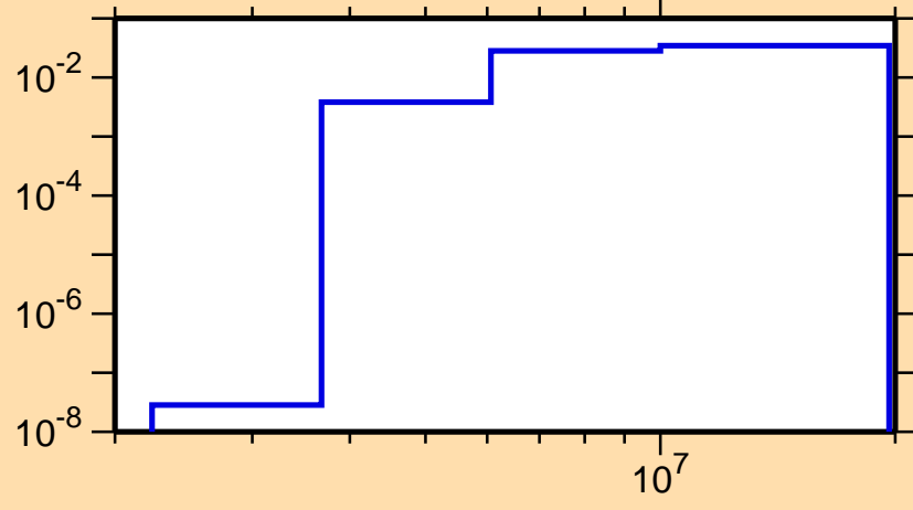
\sigma vs. E for ^{113}\text{Xe}(n,n\text{cont.})
