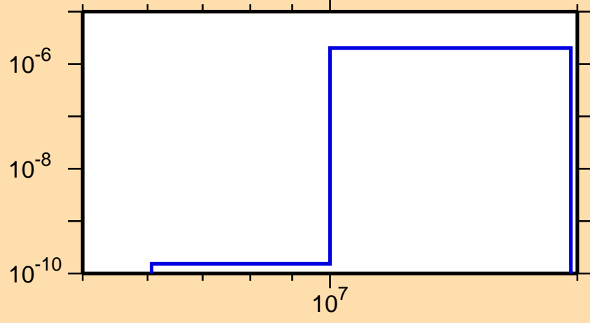
\sigma vs. E for ^{113}\text{Xe}(\text{mt117})
