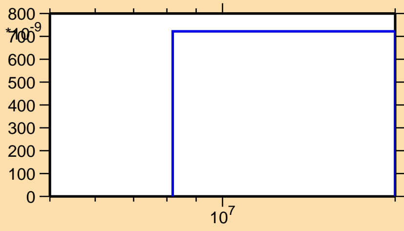
\sigma vs. E for ^{113}\text{Xe}(n,2np)
