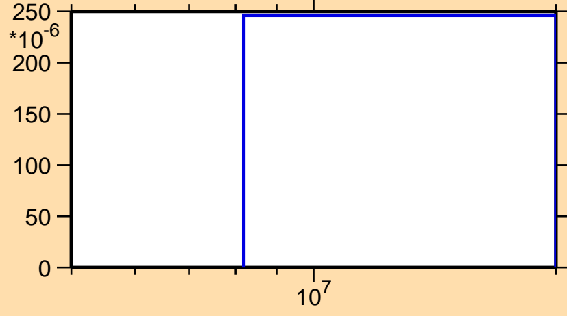
\sigma vs. E for ^{113}\text{Xe}(n,2n)
