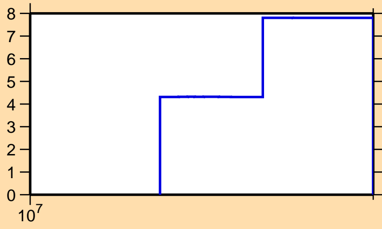
\Delta\sigma/\sigma vs. E for ^{114}\text{Xe}(n,\text{tot.})
