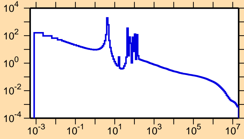
\sigma vs. E for ^{114}\text{Xe}(n,\gamma)
