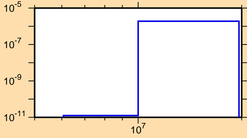
\sigma vs. E for ^{114}\text{Xe}(\text{mt117})
