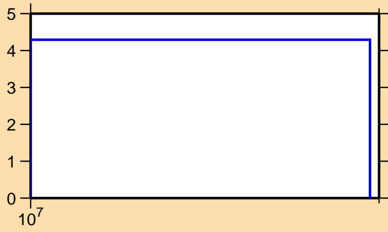
\Delta\sigma/\sigma vs. E for ^{114}\text{Xe}(n,\text{nonel.})
