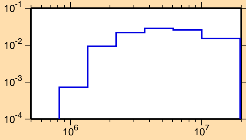
\sigma vs. E for ^{114}\text{Xe}(n,n_2)
