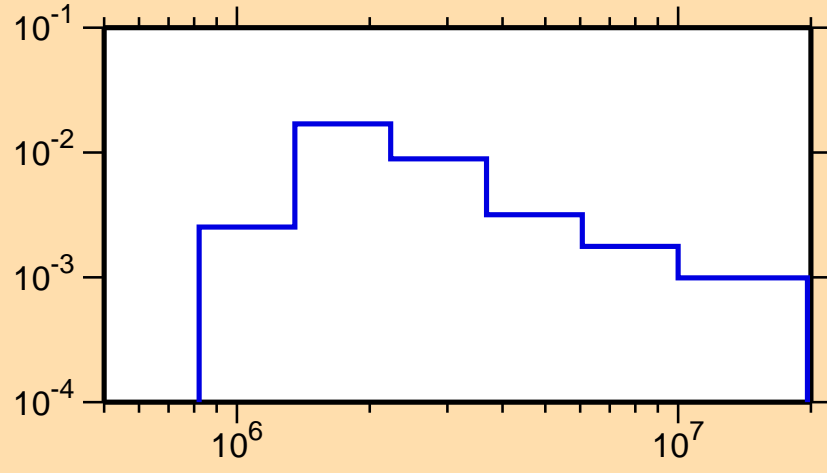
\sigma vs. E for ^{114}\text{Xe}(n,n_3)
