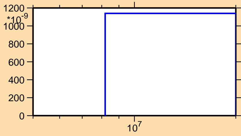
\sigma vs. E for ^{114}\text{Xe}(n,\text{pt})
