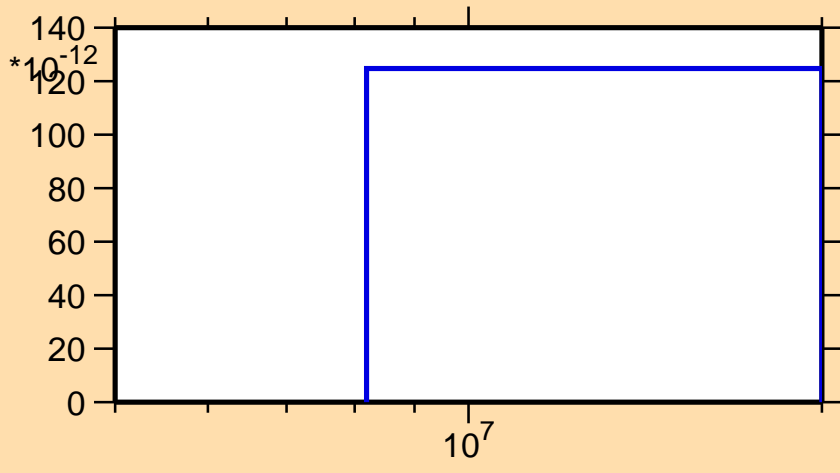
\sigma vs. E for ^{114}\text{Xe}(n,nd)
