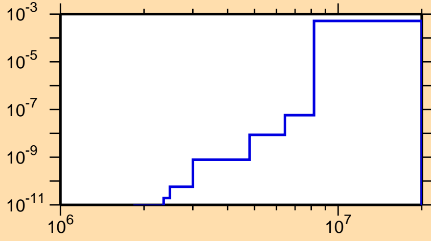
\sigma vs. E for ^{114}\text{Xe}(n,\text{He}3)
