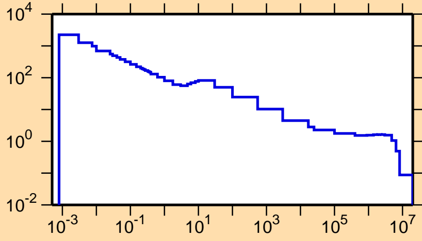
\sigma vs. E for ^{114}\text{Xe}(n,p)
