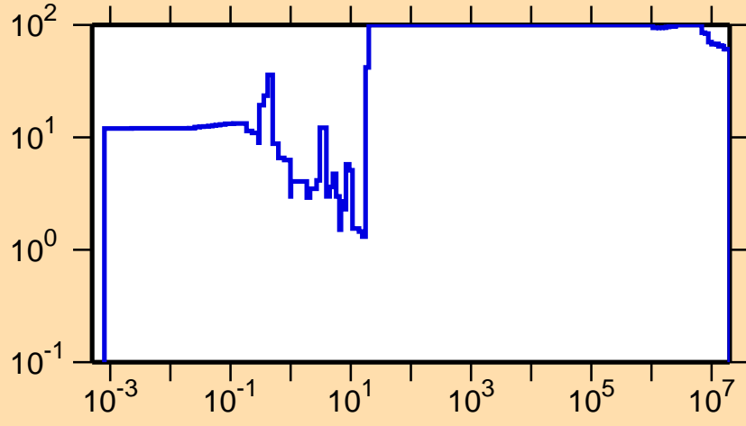
\Delta\sigma/\sigma vs. E for ^{115}\text{Xe}(n,\gamma)
