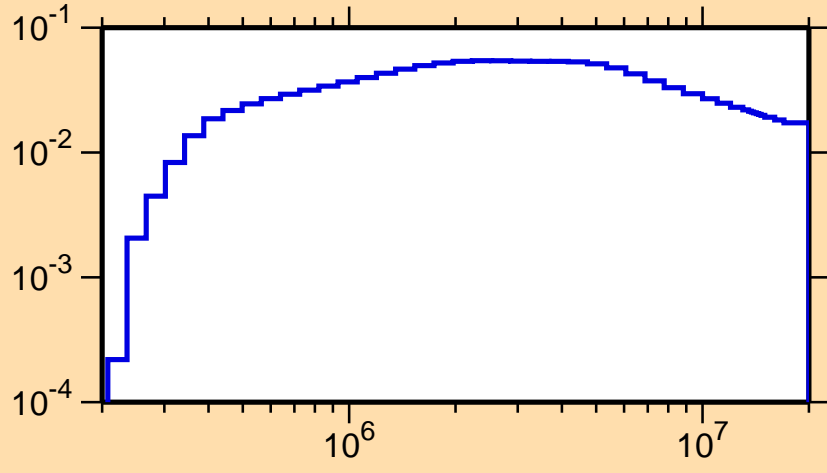
\sigma vs. E for ^{115}\text{Xe}(n,n_2)
