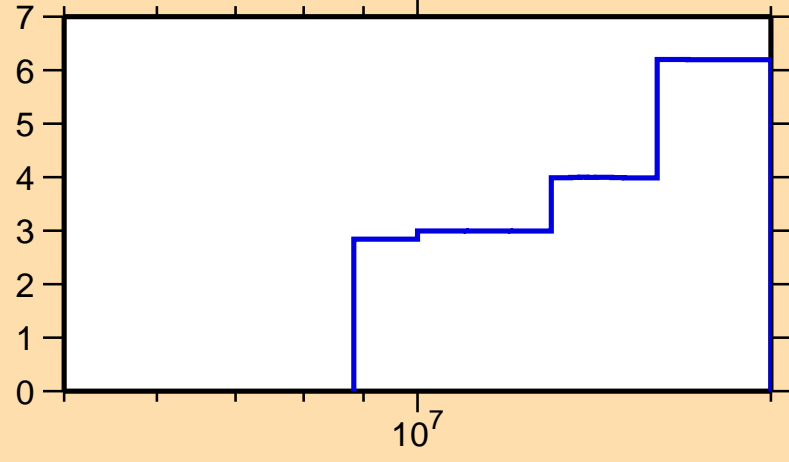
\Delta\sigma/\sigma vs. E for ^{115}\text{Xe}(n,\text{tot.})
