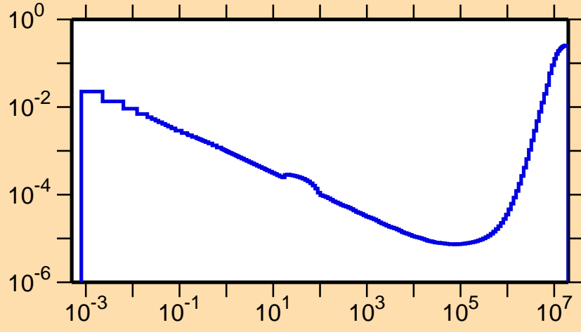
\sigma vs. E for ^{115}\text{Xe}(n,p\alpha)
