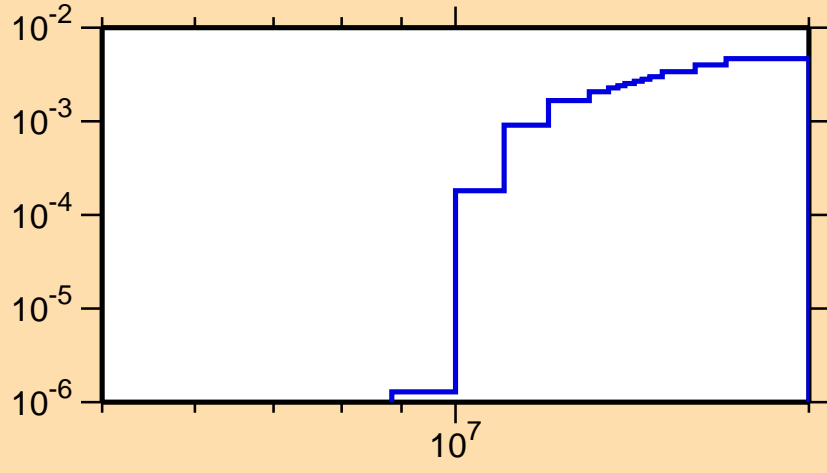
\sigma vs. E for ^{115}\text{Xe}(n,2n)
