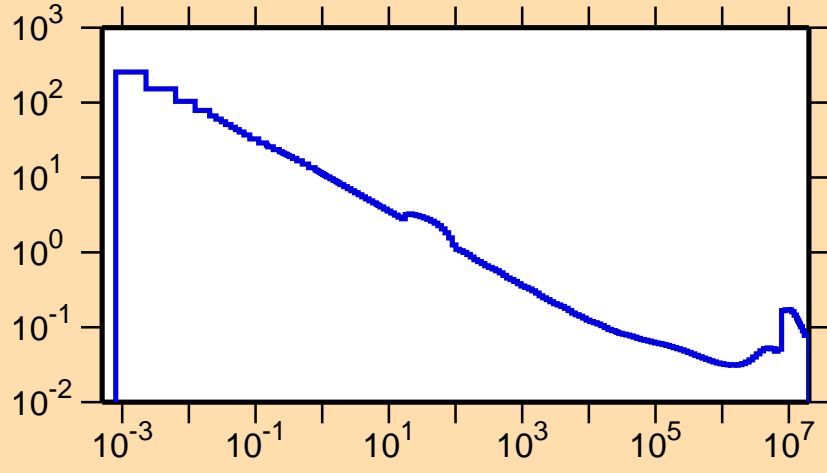
\sigma vs. E for ^{115}\text{Xe}(n,\alpha)
