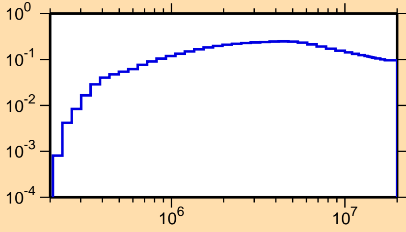
\sigma vs. E for ^{115}\text{Xe}(n,\text{inel.})
