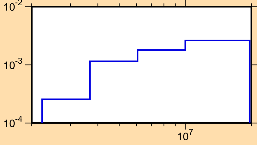
\sigma vs. E for ^{115}\text{Xe}(n,n\text{cont.})
