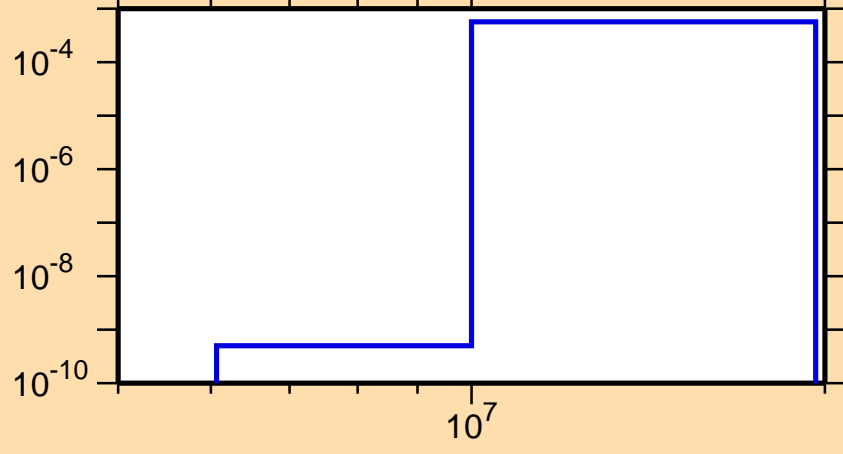
\sigma vs. E for ^{115}\text{Xe}(n,t)
