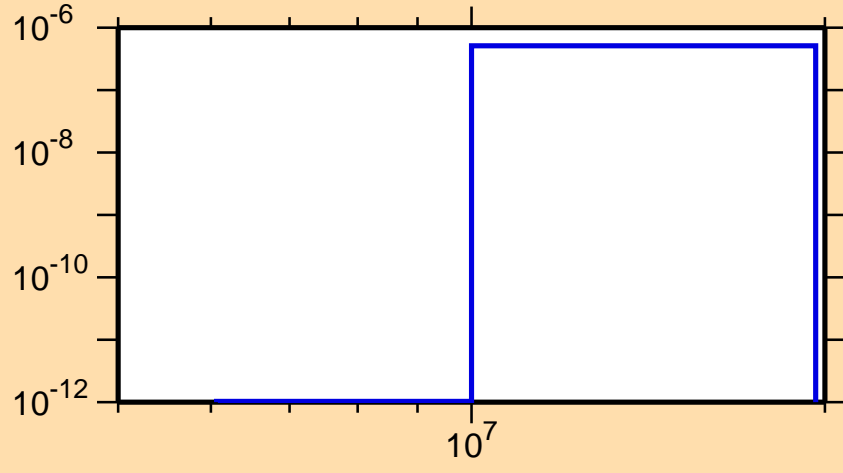
\sigma vs. E for ^{115}\text{Xe}(\text{mt117})
