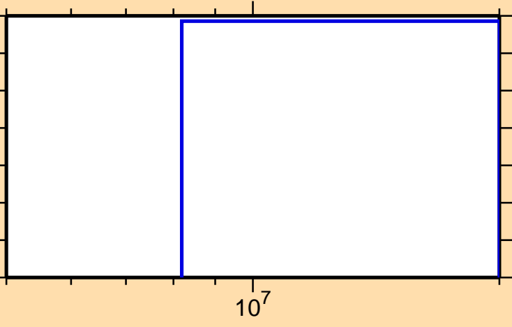
\sigma vs. E for ^{115}\text{Xe}(\text{mt } 34)
