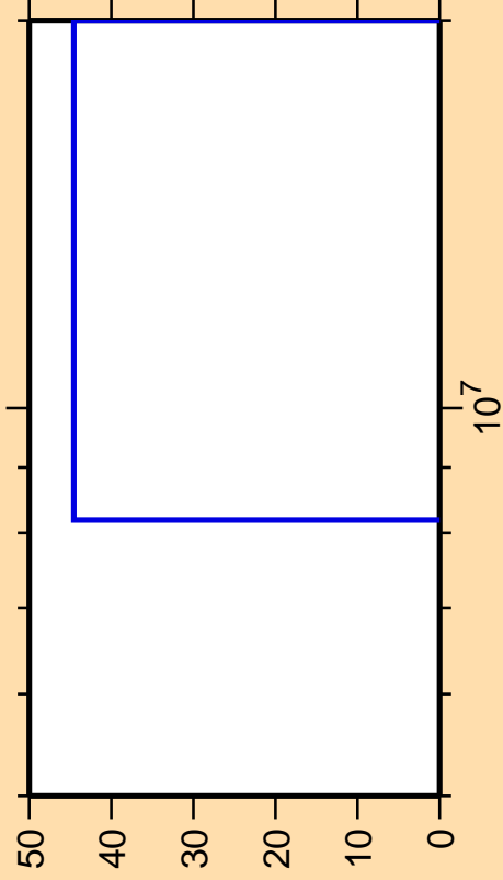
\Delta\sigma/\sigma vs. E for ^{115}\text{Xe}(n,n_1)
