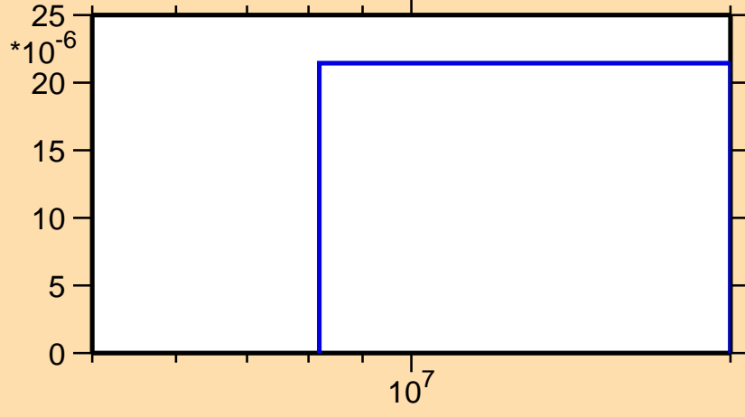
\sigma vs. E for ^{115}\text{Xe}(n,\text{pt})
