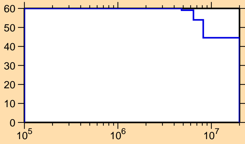
\Delta\sigma/\sigma vs. E for ^{115}\text{Xe}(n,n_1)
