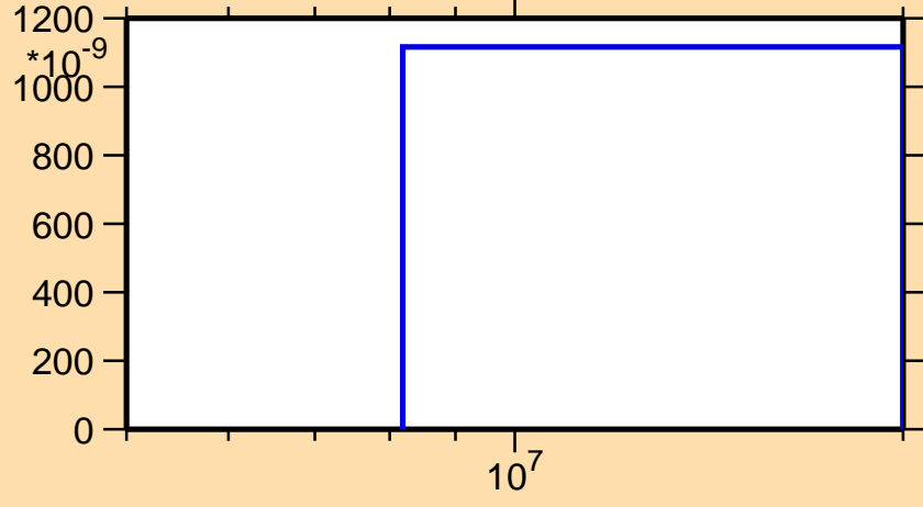
\sigma vs. E for ^{115}\text{Xe}(n,2n\alpha)
