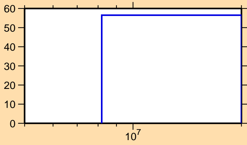
\Delta\sigma/\sigma vs. E for ^{115}\text{Xe}(n,2n)
