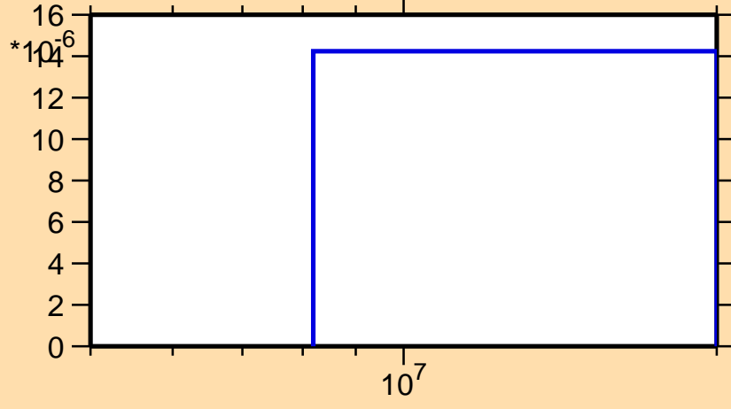
\sigma vs. E for ^{115}\text{Xe}(\text{mt } 45)
