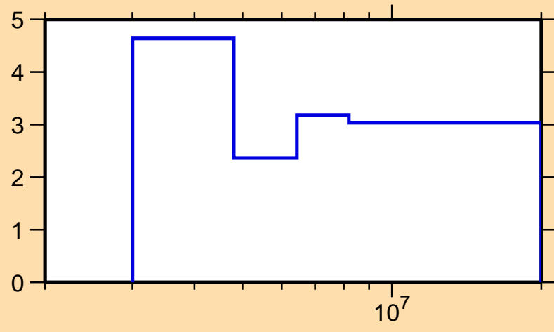
\Delta\sigma/\sigma vs. E for ^{116}\text{Xe}(n,\text{nonel.})
