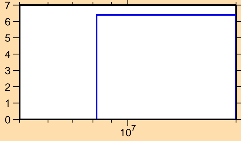
\Delta\sigma/\sigma vs. E for ^{116}\text{Xe}(n,\text{el.})
