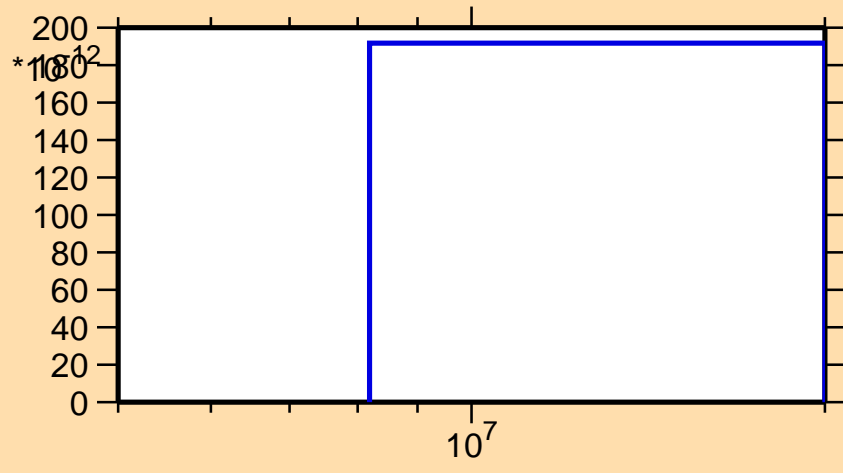
\sigma vs. E for ^{116}\text{Xe}(n,nd)
