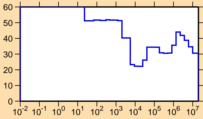
\Delta\sigma/\sigma vs. E for ^{117}\text{Xe}(n,p)
