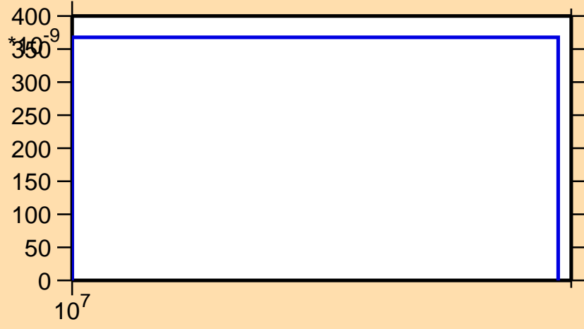
\sigma vs. E for ^{117}\text{Xe}(n,\text{nd})
