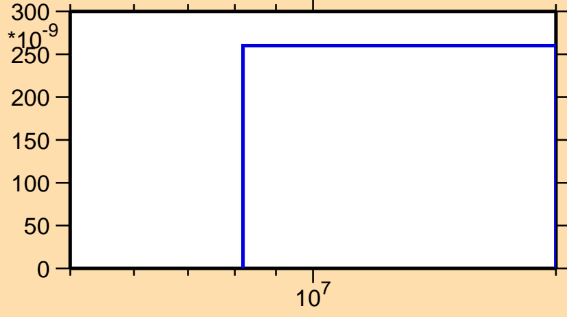
\sigma vs. E for ^{117}\text{Xe}(n,2n\alpha)
