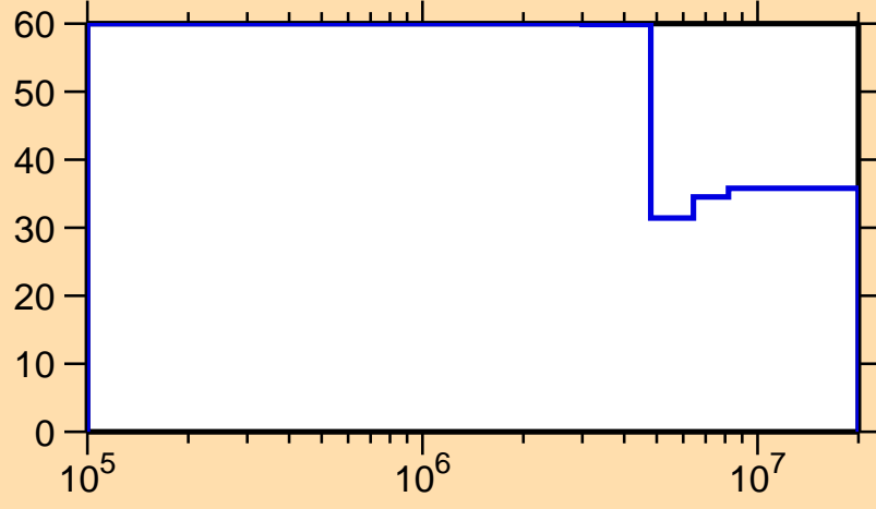
\Delta\sigma/\sigma vs. E for ^{117}\text{Xe}(n,n_1)
