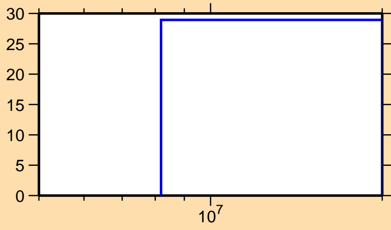
\Delta\sigma/\sigma vs. E for ^{117}\text{Xe}(n,\text{inel.})
