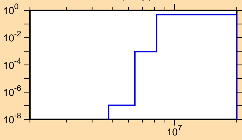
\sigma vs. E for ^{117}\text{Xe}(n,np)
