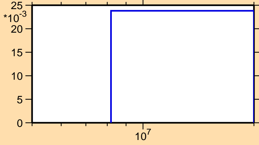
\sigma vs. E for ^{117}\text{Xe}(n,2n)
