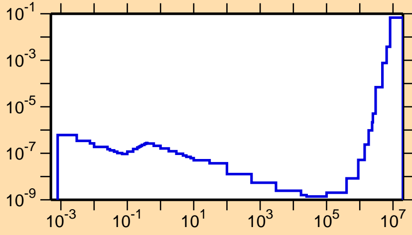
\sigma vs. E for ^{117}\text{Xe}(n,p\alpha)
