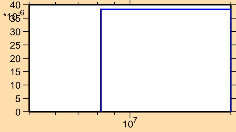
\sigma vs. E for ^{117}\text{Xe}(n,\text{pd})
