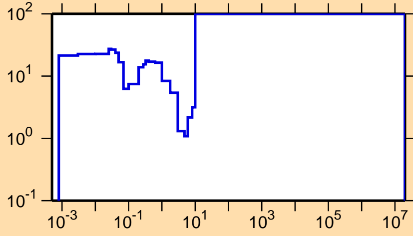
\Delta\sigma/\sigma vs. E for ^{117}\text{Xe}(n,\gamma)
