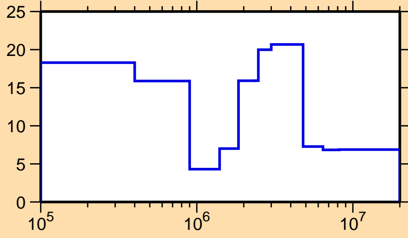
\Delta\sigma/\sigma vs. E for ^{117}\text{Xe}(n,\text{el.})
