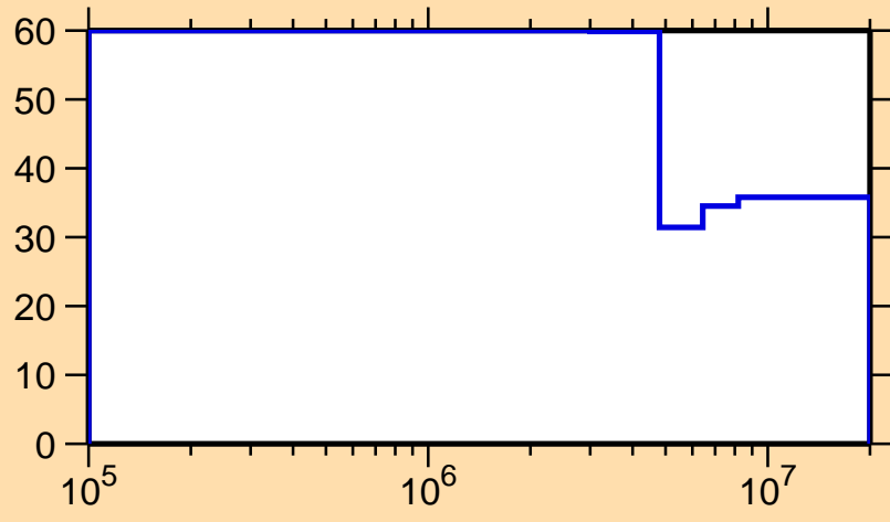
\Delta\sigma/\sigma vs. E for ^{117}\text{Xe}(n,n_1)
