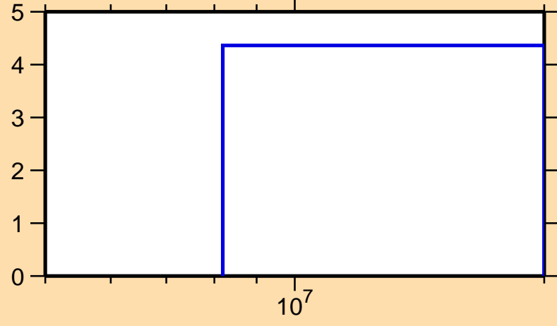
\Delta\sigma/\sigma vs. E for ^{117}\text{Xe}(n,\text{tot.})
