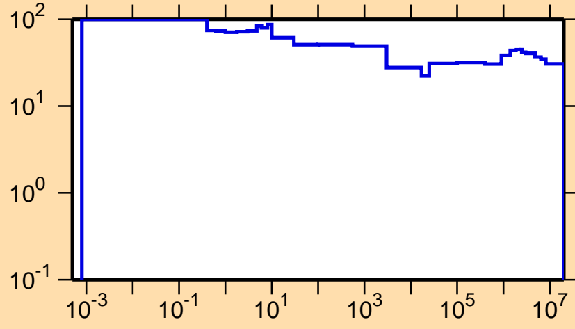
\Delta\sigma/\sigma vs. E for ^{117}\text{Xe}(n,p)
