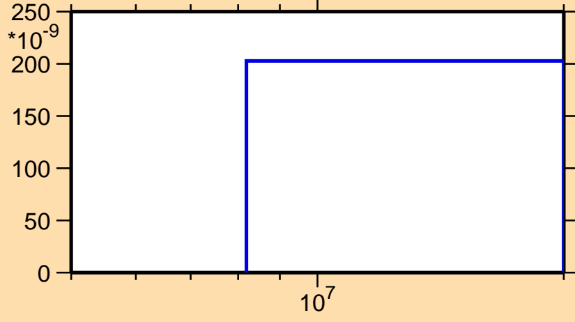
\sigma vs. E for ^{117}\text{Xe}(\text{mt117})
