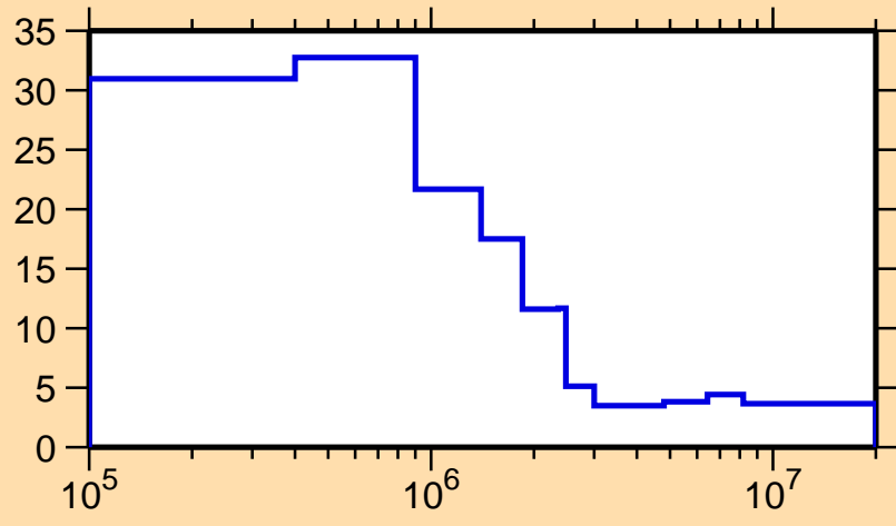
\Delta\sigma/\sigma vs. E for ^{117}\text{Xe}(n,\text{nonel.})
