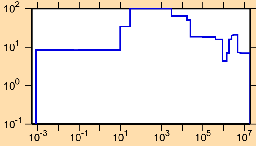
\Delta\sigma/\sigma vs. E for ^{117}\text{Xe}(n,\text{el.})
