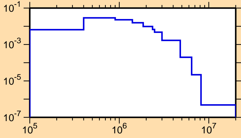
\sigma vs. E for ^{117}\text{Xe}(n,n_3)
