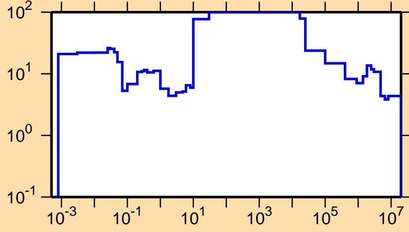
\Delta\sigma/\sigma vs. E for ^{117}\text{Xe}(n,\text{tot.})
