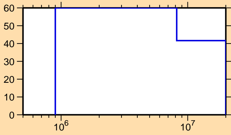
\Delta\sigma/\sigma vs. E for ^{117}\text{Xe}(n,n\text{cont.})
