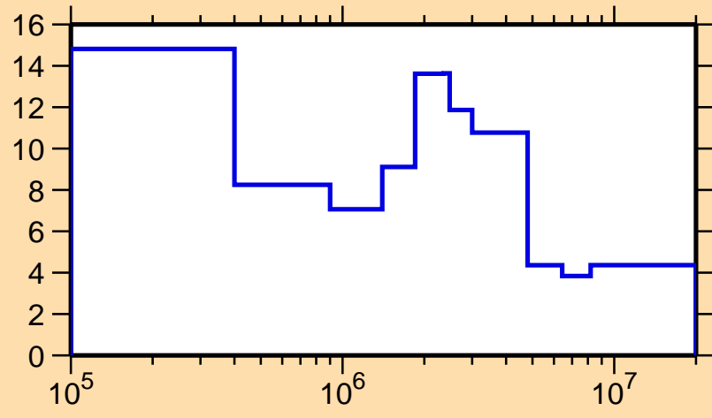
\Delta\sigma/\sigma vs. E for ^{117}\text{Xe}(n,\text{tot.})
