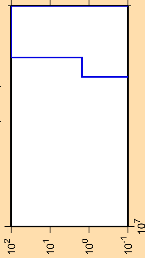
\Delta\sigma/\sigma vs. E for ^{118}\text{Xe} (mt 34)
