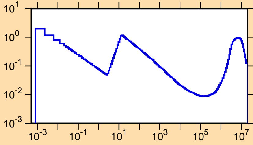
\sigma vs. E for ^{118}\text{Xe}(n,p)
