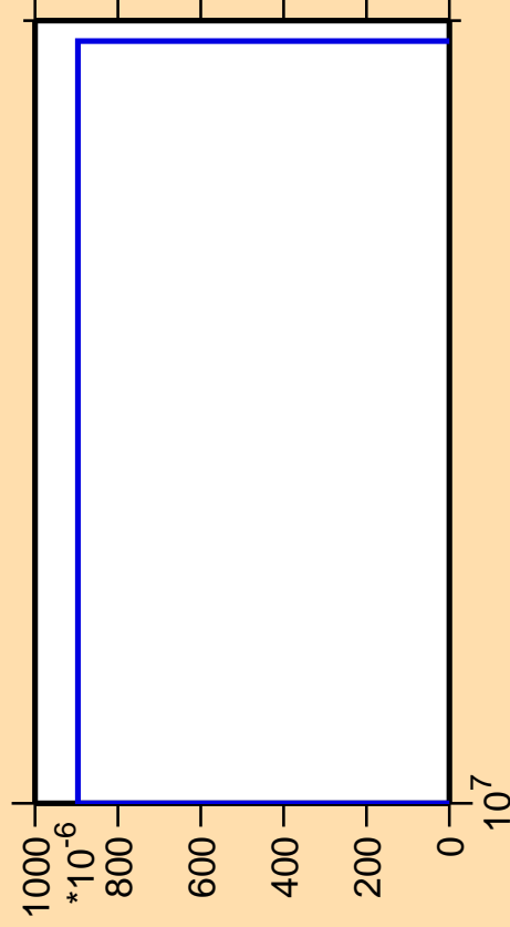
\Delta\sigma/\sigma vs. E for ^{118}\text{Xe}(n,nt)
