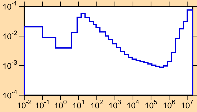
\sigma vs. E for ^{118}\text{Xe}(n,\alpha)
