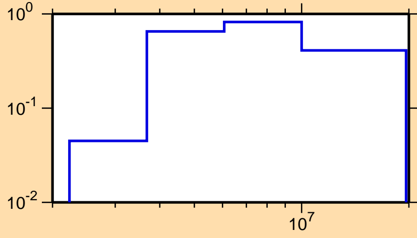
\sigma vs. E for ^{118}\text{Xe}(n,n\text{cont.})
