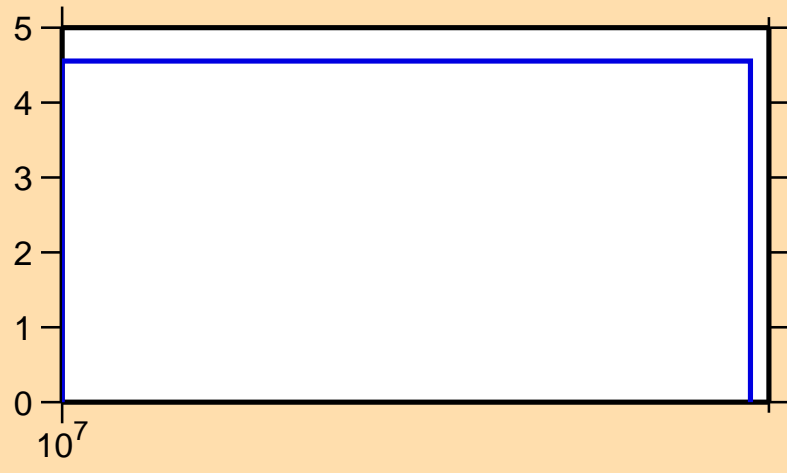
\Delta\sigma/\sigma vs. E for ^{118}\text{Xe}(n,\text{tot.})
