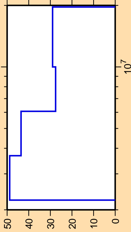
\Delta\sigma/\sigma vs. E for ^{118}\text{Xe}(n,n\text{cont.})
