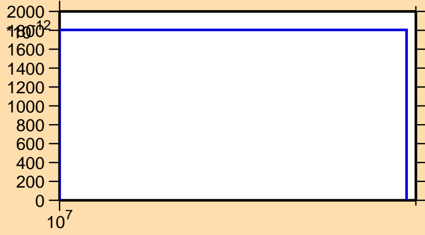
\sigma vs. E for ^{118}\text{Xe}(n,2np)
