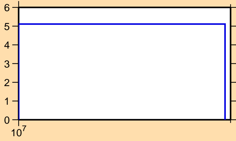
\Delta\sigma/\sigma vs. E for ^{118}\text{Xe}(n,\text{el.})
