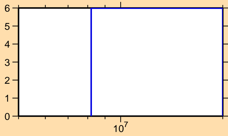
\Delta\sigma/\sigma vs. E for ^{118}\text{Xe}(n,\text{nonel.})
