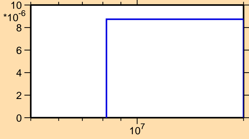
\sigma vs. E for ^{118}\text{Xe}(n,\text{pd})
