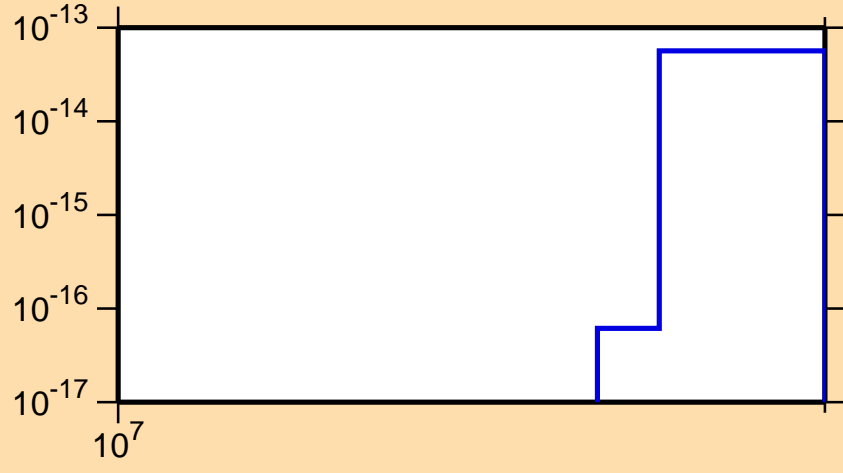
\sigma vs. E for ^{119}\text{Xe}(n,nt)
