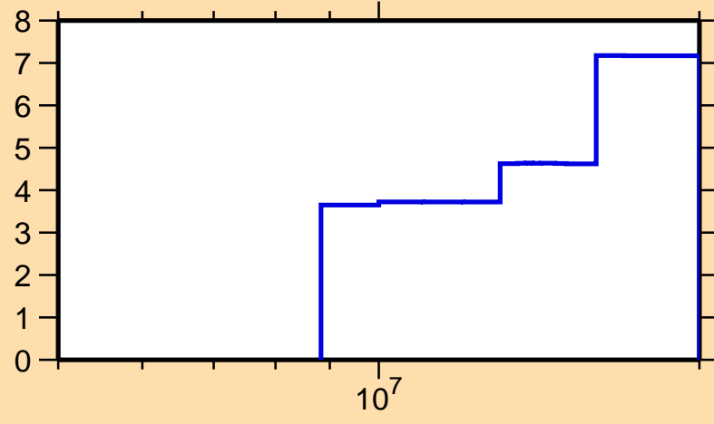
\Delta\sigma/\sigma vs. E for ^{119}\text{Xe}(n,\text{el.})
