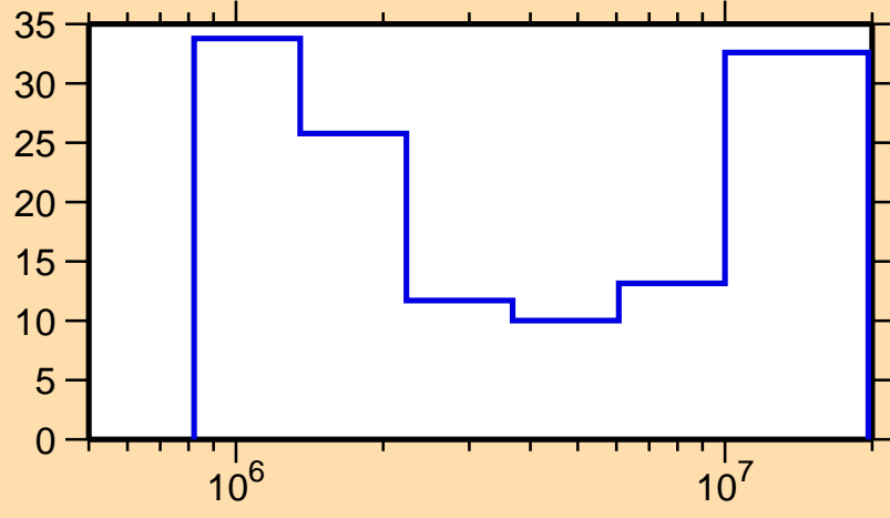
\Delta\sigma/\sigma vs. E for ^{119}\text{Xe}(n,n\text{cont.})
