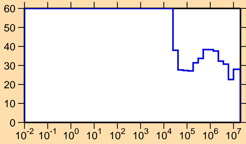
\Delta\sigma/\sigma vs. E for ^{119}\text{Xe}(n,p)
