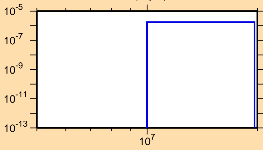
\sigma vs. E for ^{119}\text{Xe}(n,pd)
