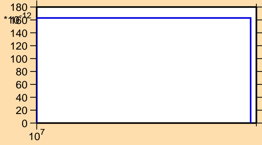
\sigma vs. E for ^{119}\text{Xe} (mt 34)
