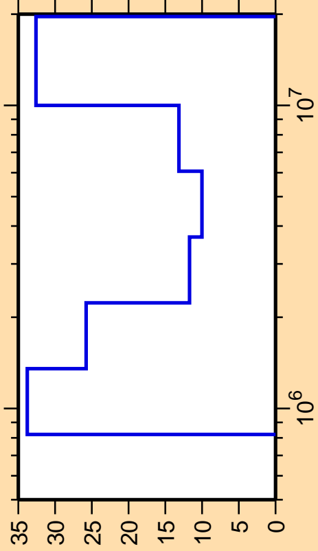
\Delta\sigma/\sigma vs. E for ^{119}\text{Xe}(n,\text{ncont.})
