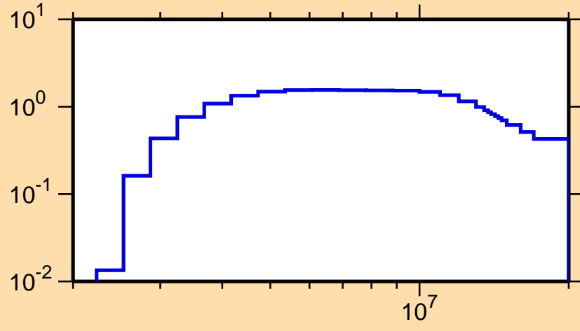
\sigma vs. E for ^{120}\text{Xe}(n,n\text{cont.})
