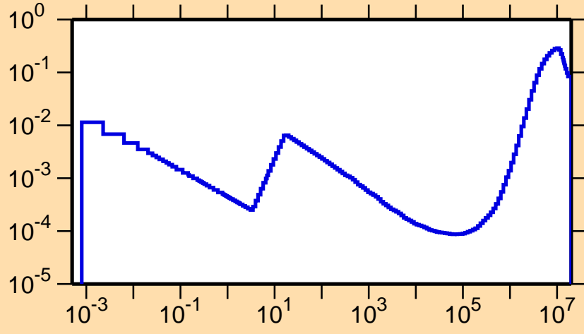
\sigma vs. E for ^{120}\text{Xe}(n,p)
