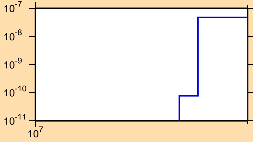
\sigma vs. E for ^{120}\text{Xe}(n,2n\alpha)
