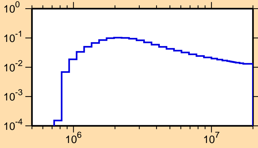
\sigma vs. E for ^{120}\text{Xe}(n,n_2)
