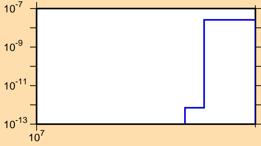
\sigma vs. E for ^{120}\text{Xe}(n,\text{nd})
