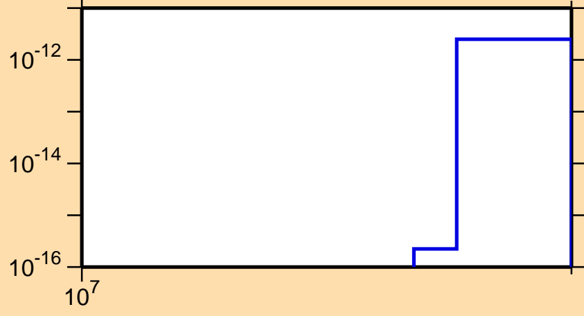
\sigma vs. E for ^{120}\text{Xe} (mt 34)
