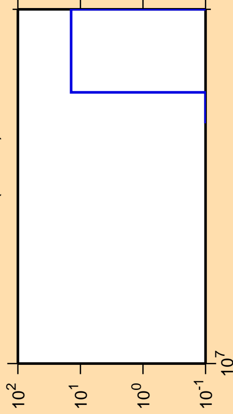
\Delta\sigma/\sigma vs. E for ^{120}\text{Xe} (mt 34)
