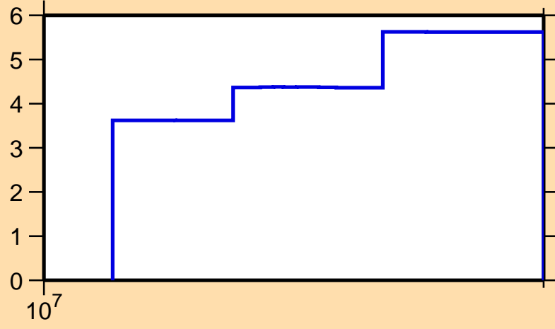
\Delta\sigma/\sigma vs. E for ^{120}\text{Xe}(n,\text{el.})
