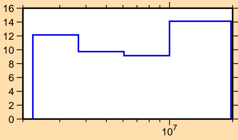
\Delta\sigma/\sigma vs. E for ^{120}\text{Xe}(n,n\text{cont.})
