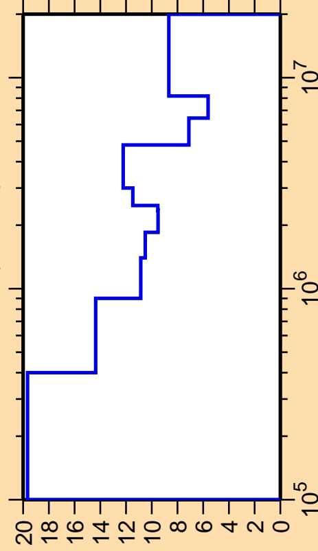
\Delta\sigma/\sigma vs. E for ^{120}\text{Xe}(n,\text{inel.})
