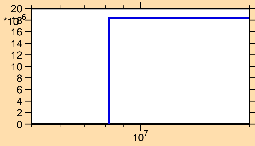
\sigma vs. E for ^{120}\text{Xe}(n,t)
