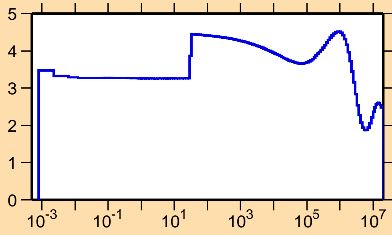
\sigma vs. E for ^{121}\text{Xe}(n,\text{el.})
