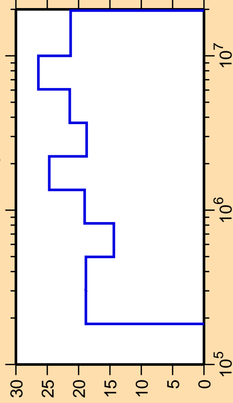
\Delta\sigma/\sigma vs. E for ^{121}\text{Xe}(n,n_3)
