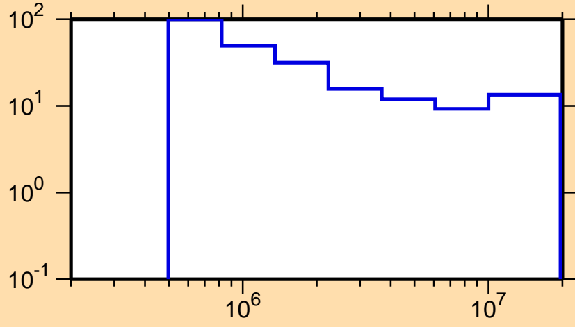
\Delta\sigma/\sigma vs. E for ^{121}\text{Xe}(n,n\text{cont.})
