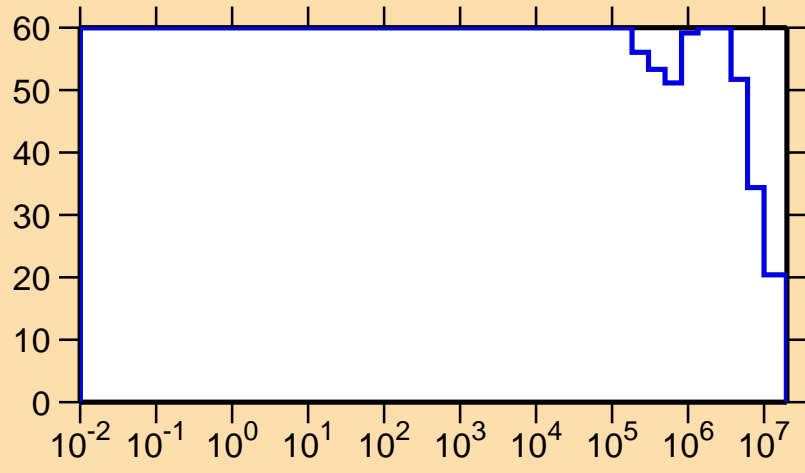
\Delta\sigma/\sigma vs. E for ^{121}\text{Xe}(n,p)
