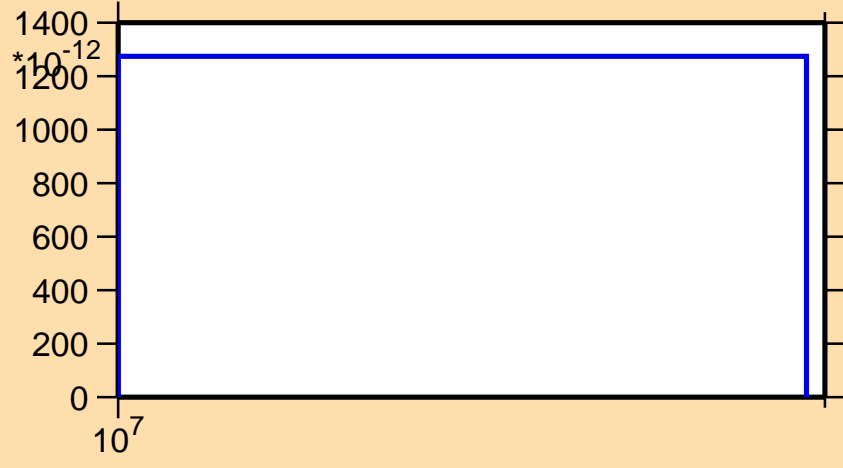
\sigma vs. E for ^{121}\text{Xe}(n,\text{pt})
