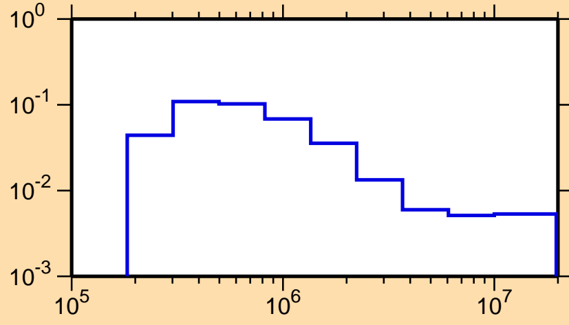
\sigma vs. E for ^{121}\text{Xe}(n,n_3)
