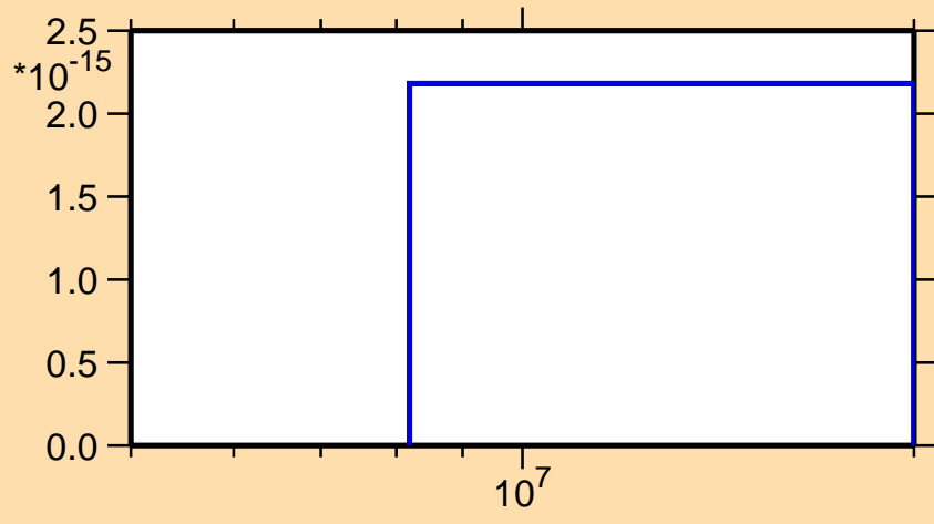
\sigma vs. E for ^{121}\text{Xe}(n,3n)
