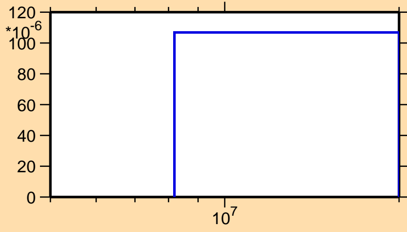
\sigma vs. E for ^{121}\text{Xe}(n,t)
