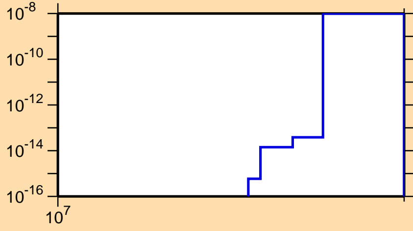
\sigma vs. E for ^{122}\text{Xe}(n,\text{nd})
