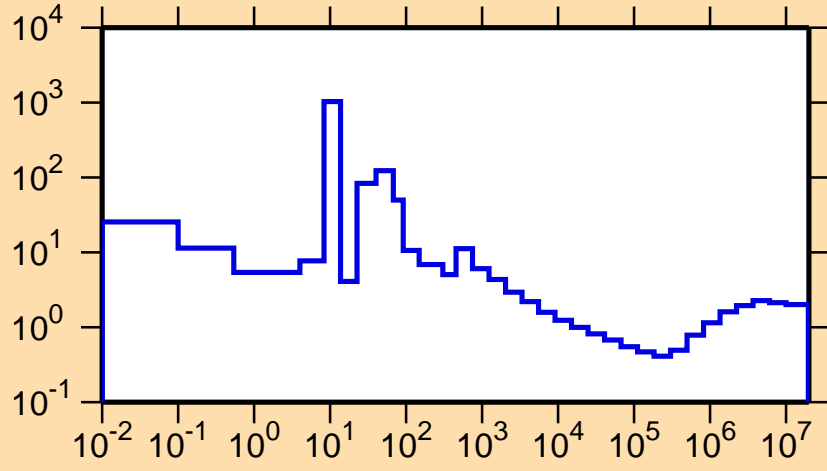
\sigma vs. E for ^{122}\text{Xe}(n,\text{nonel.})
