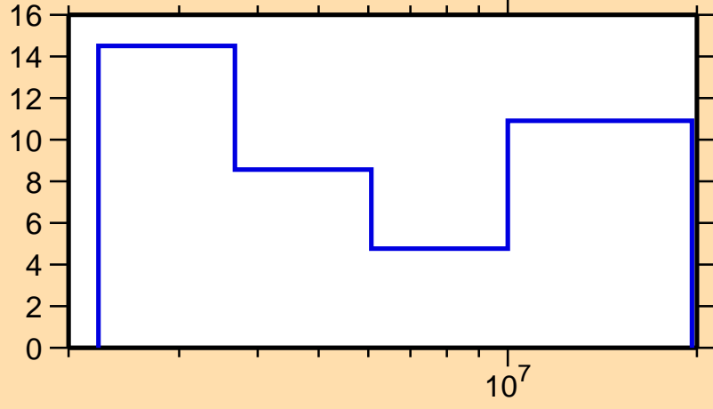
\Delta\sigma/\sigma vs. E for ^{122}\text{Xe}(n,n\text{cont.})
