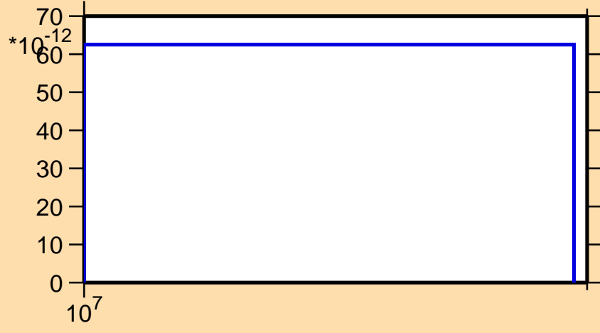
\sigma vs. E for ^{122}\text{Xe}(n,nd)
