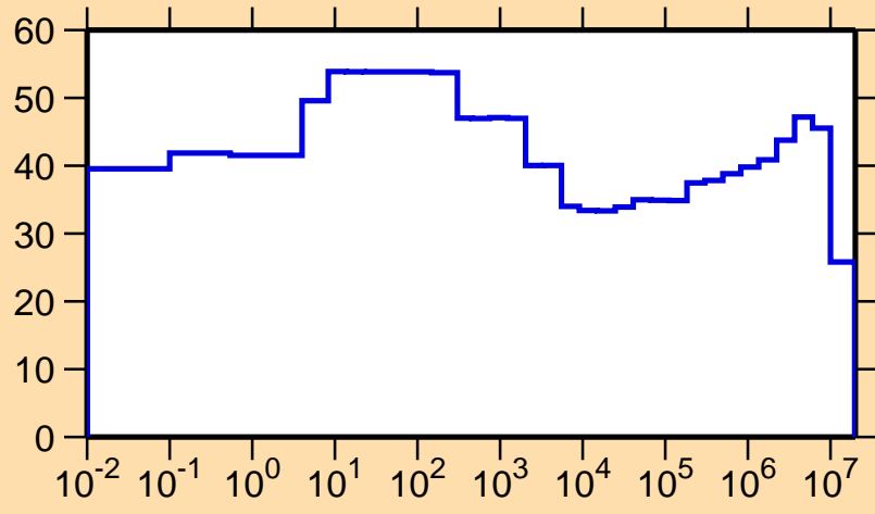
\Delta\sigma/\sigma vs. E for ^{122}\text{Xe}(n,p)
