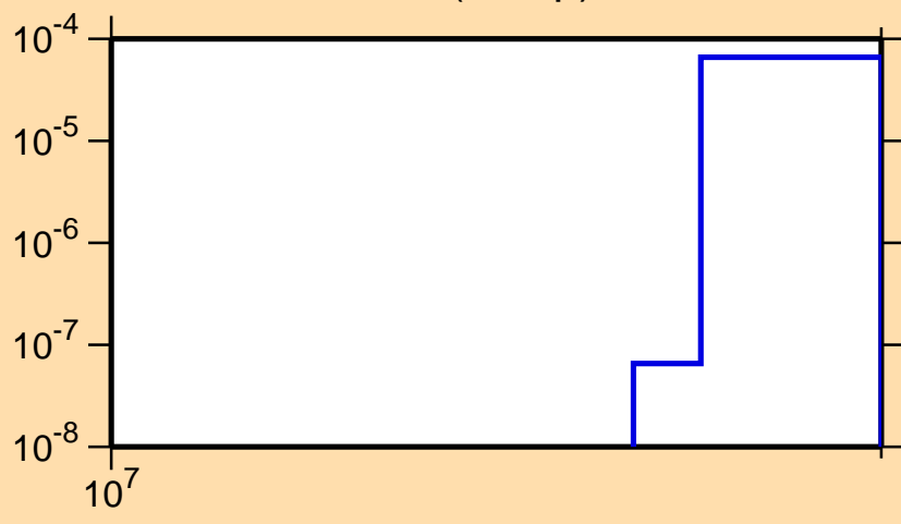
\sigma vs. E for ^{123}\text{Xe}(n,2np)
