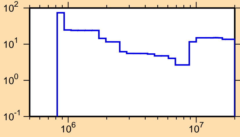
\Delta\sigma/\sigma vs. E for ^{123}\text{Xe}(n,n\text{cont.})
