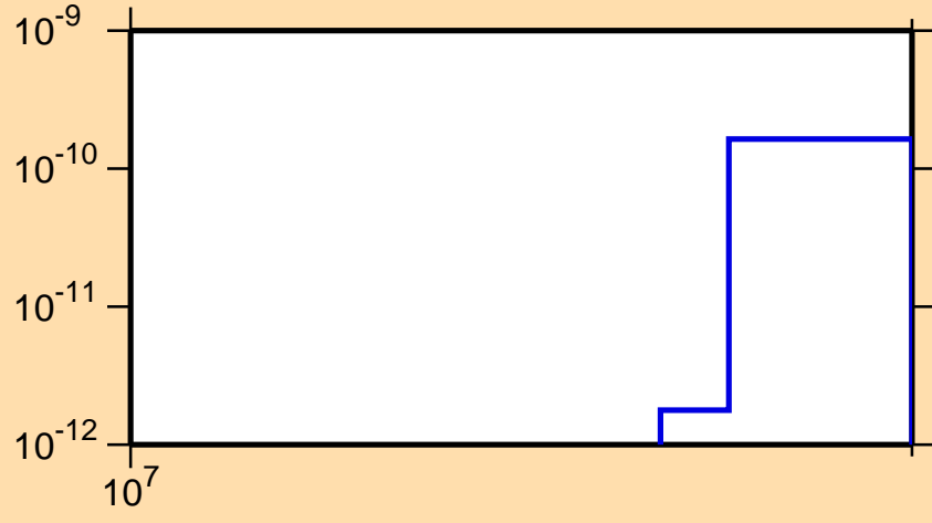
\sigma vs. E for ^{123}\text{Xe}(\text{mt } 45)
