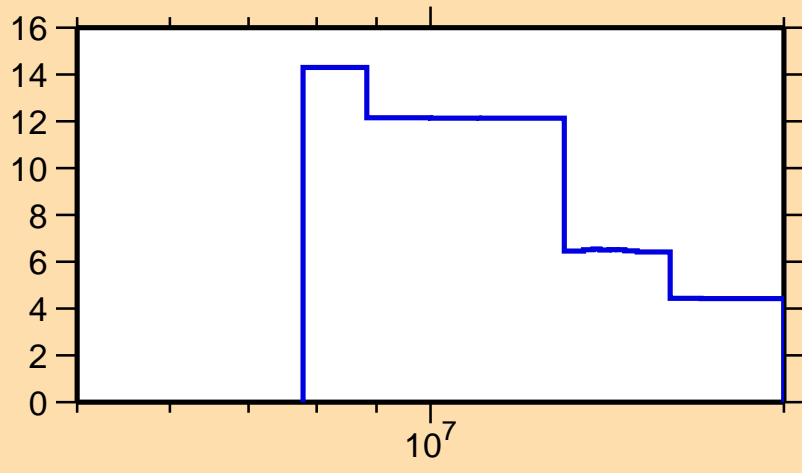
\Delta\sigma/\sigma vs. E for ^{123}\text{Xe}(n,2n)
