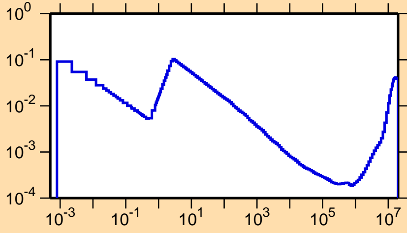
\sigma vs. E for ^{123}\text{Xe}(n,\alpha)
