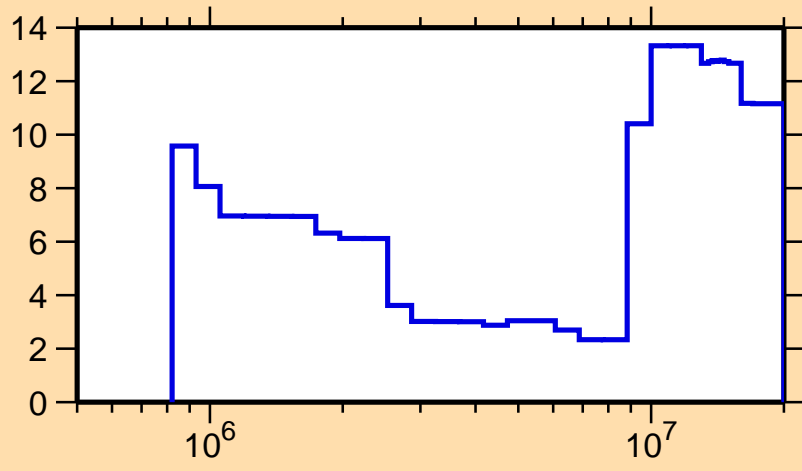
\Delta\sigma/\sigma vs. E for ^{123}\text{Xe}(n,\text{inel.})
