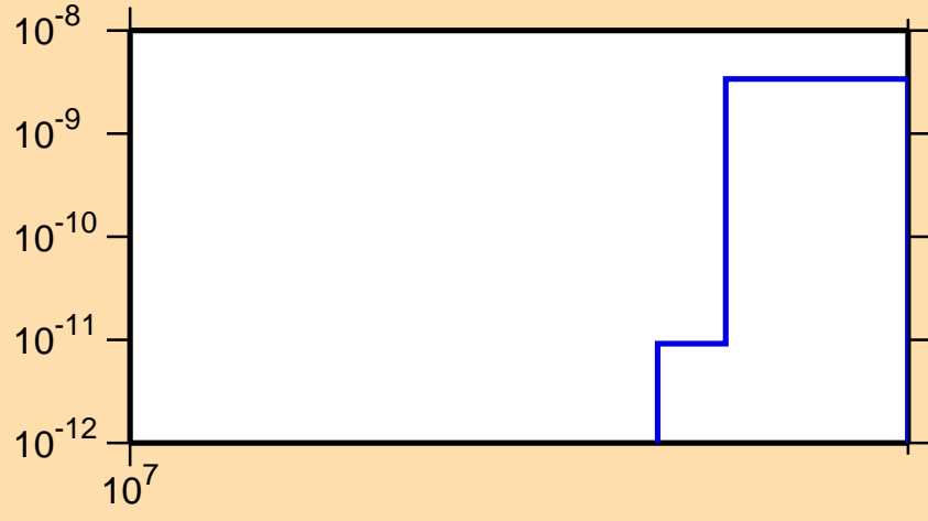
\sigma vs. E for ^{123}\text{Xe}(n,\text{pt})
