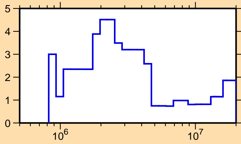
\Delta\sigma/\sigma vs. E for ^{123}\text{Xe}(n,\text{tot.})
