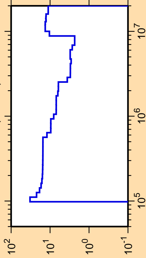
\Delta\sigma/\sigma vs. E for ^{123}\text{Xe}(n,\text{inel.})
