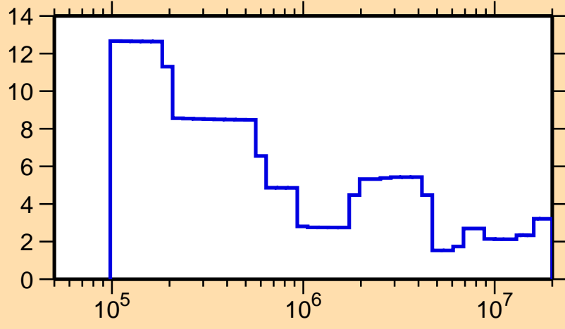
\Delta\sigma/\sigma vs. E for ^{123}\text{Xe}(n,\text{el.})
