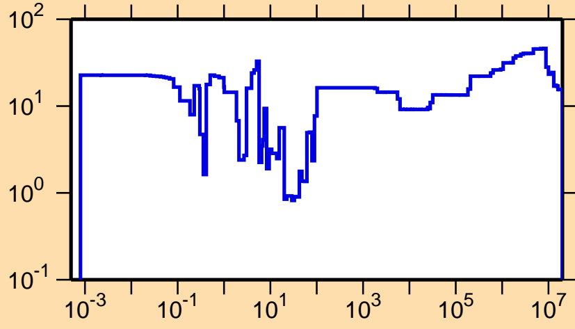
\Delta\sigma/\sigma vs. E for ^{123}\text{Xe}(n,\gamma)
