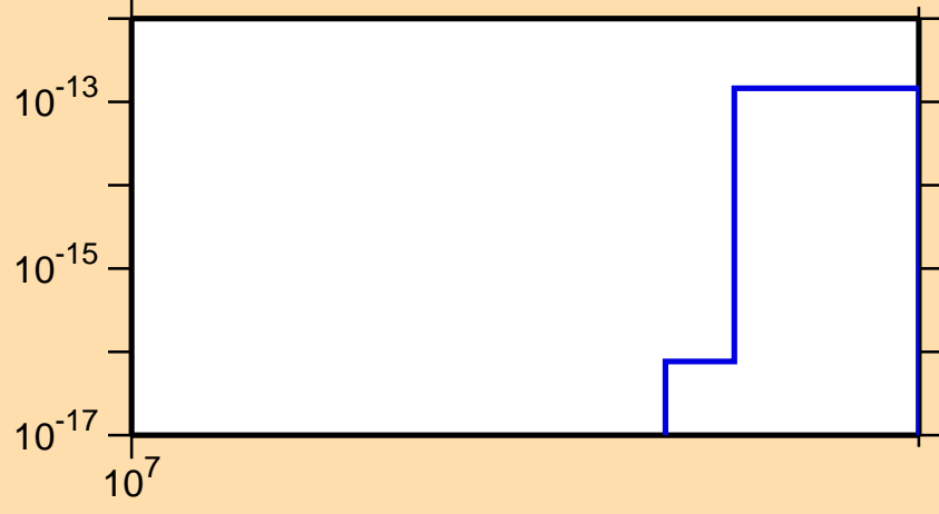
\sigma vs. E for ^{123}\text{Xe}(n,nt)
