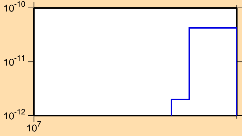
\sigma vs. E for ^{123}\text{Xe}(\text{mt117})
