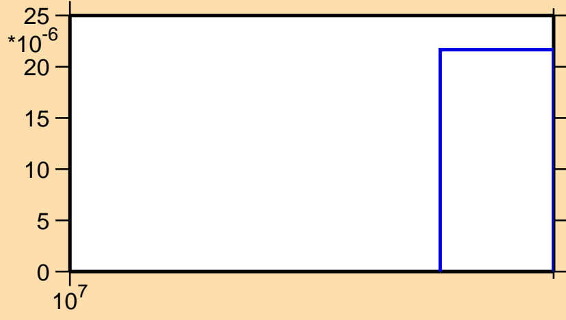
\sigma vs. E for ^{123}\text{Xe}(n,3n)
