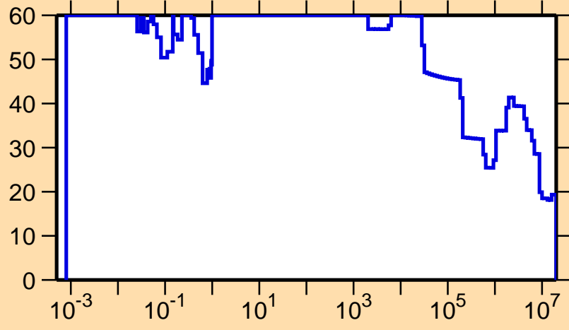
\Delta\sigma/\sigma vs. E for ^{123}\text{Xe}(n,p)
