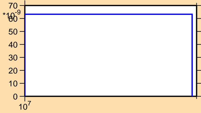
\sigma vs. E for ^{123}\text{Xe}(n,2n\alpha)
