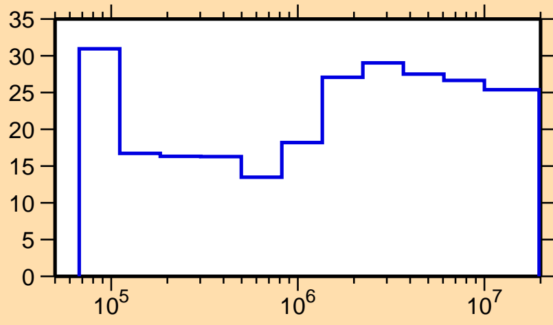
\Delta\sigma/\sigma vs. E for ^{123}\text{Xe}(n,n_1)
