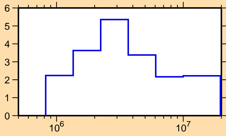
\Delta\sigma/\sigma vs. E for ^{123}\text{Xe}(n, el.)
