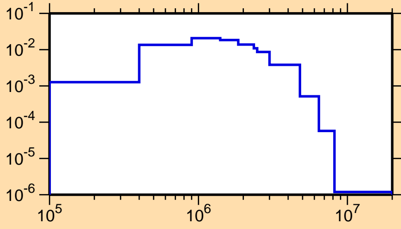
\sigma vs. E for ^{123}\text{Xe}(n,n_4)
