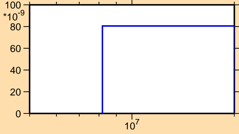
\sigma vs. E for ^{123}\text{Xe}(n,\text{nd})
