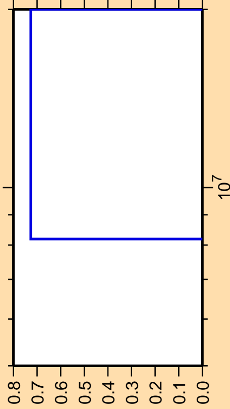
\Delta\sigma/\sigma vs. E for ^{123}\text{Xe}(\text{mt } 34)
