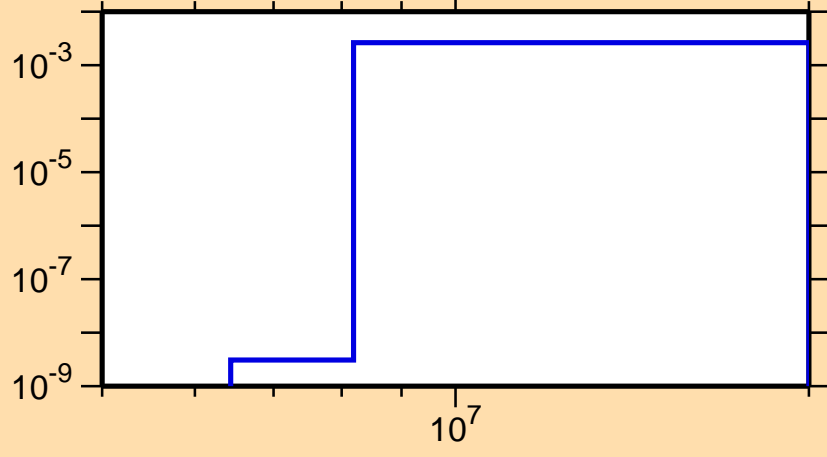
\sigma vs. E for ^{123}\text{Xe}(n,d)
