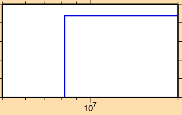
\sigma vs. E for ^{123}\text{Xe}(n,\text{He}3)
