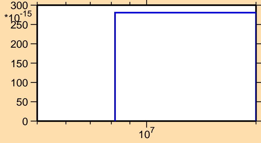
\sigma vs. E for ^{123}\text{Xe}(\text{mt } 34)
