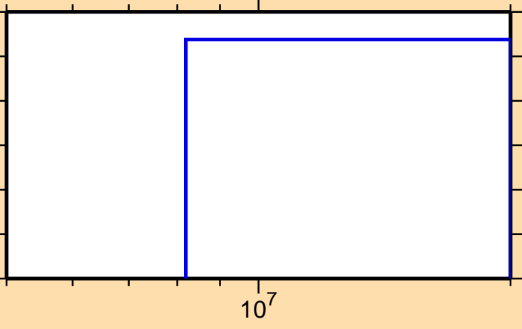
\sigma vs. E for ^{123}\text{Xe}(n,2n\alpha)
