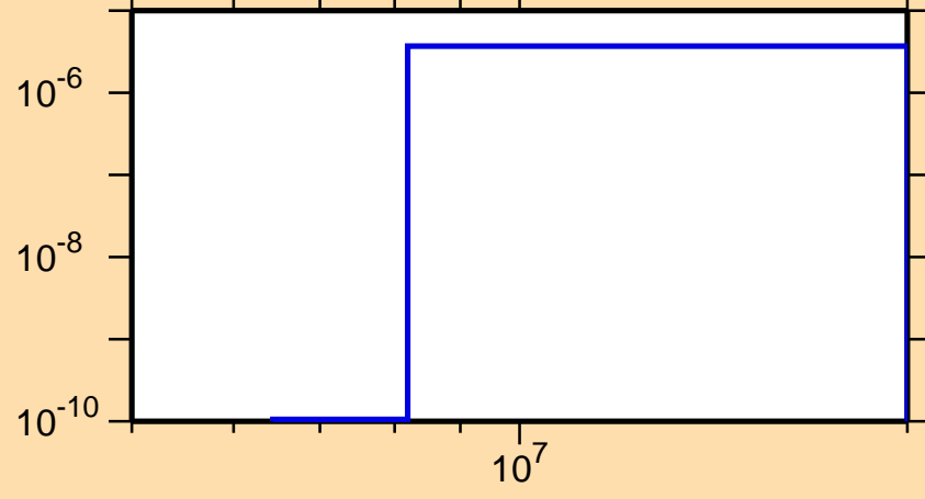
\sigma vs. E for ^{123}\text{Xe}(n,p\alpha)
