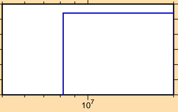
\sigma vs. E for ^{123}\text{Xe}(n,2np)
