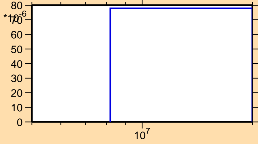
\sigma vs. E for ^{123}\text{Xe}(n,t)
