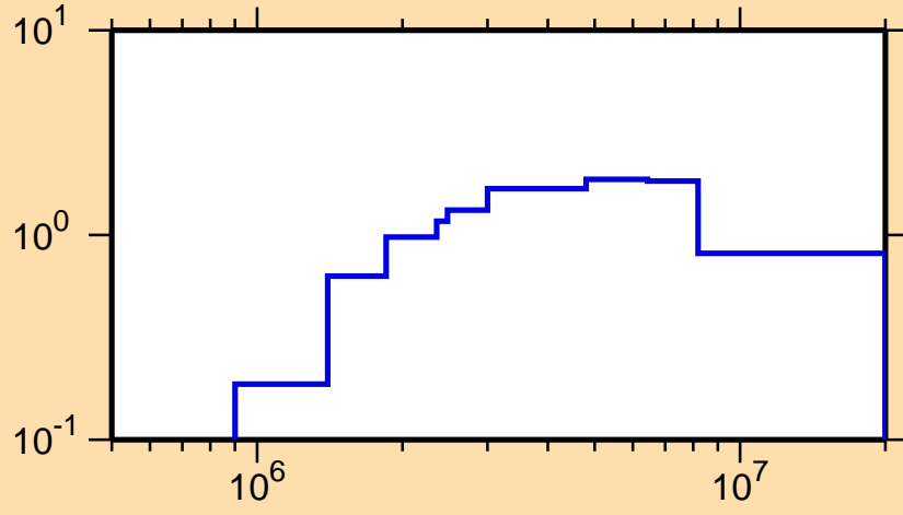
\sigma vs. E for ^{123}\text{Xe}(n,n\text{cont.})
