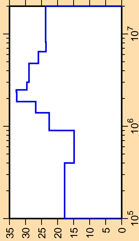
\Delta\sigma/\sigma vs. E for ^{123}\text{Xe}(n,n_4)
