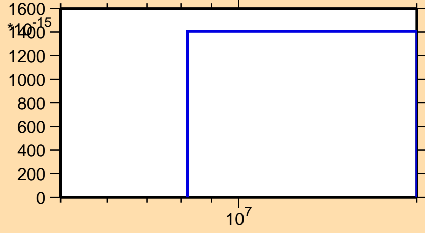
\sigma vs. E for ^{123}\text{Xe}(\text{mt } 45)
