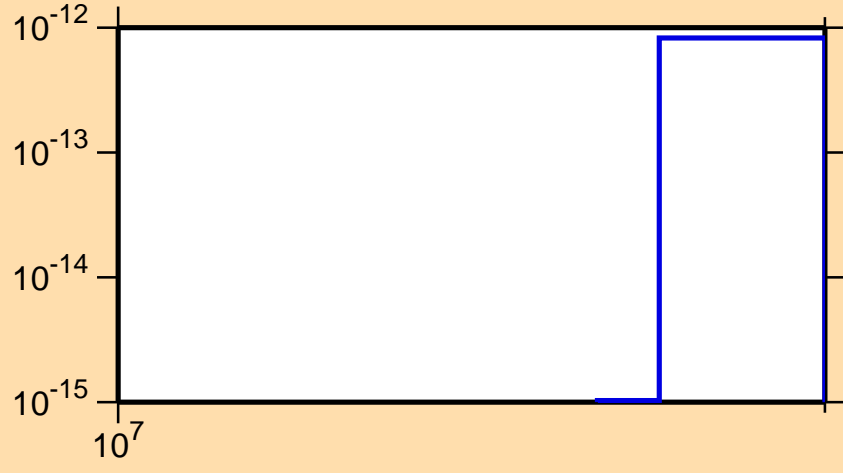
\sigma vs. E for ^{124}\text{Xe}(n,nt)
