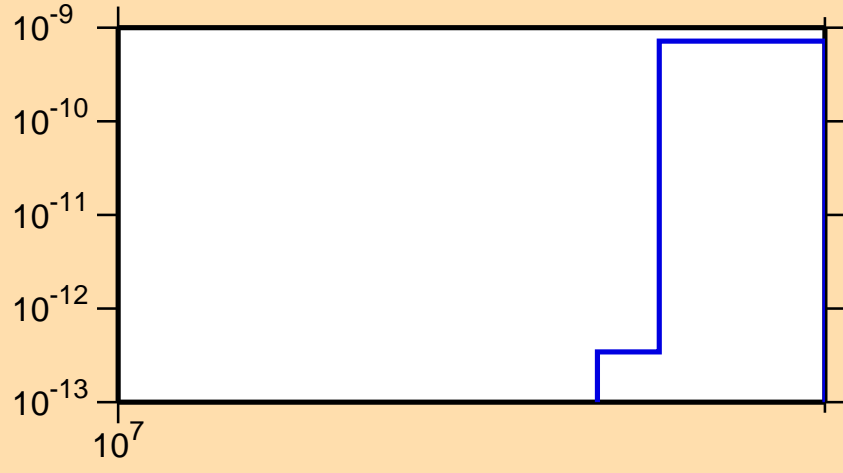
\sigma vs. E for ^{124}\text{Xe}(n,2n\alpha)
