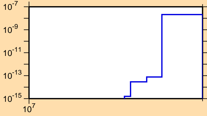
\sigma vs. E for ^{124}\text{Xe}(n,\text{nd})
