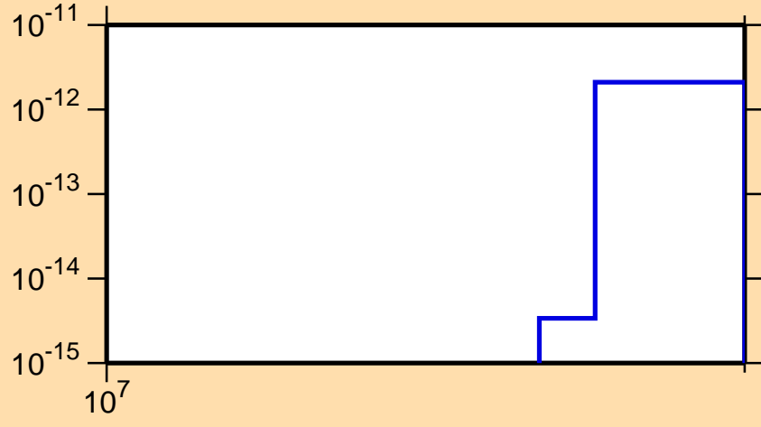
\sigma vs. E for ^{124}\text{Xe}(\text{mt } 45)
