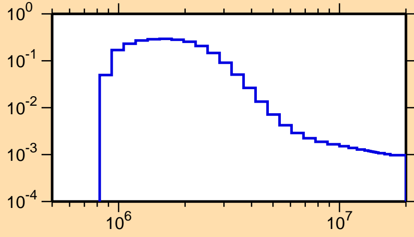
\sigma vs. E for ^{124}\text{Xe}(n,n_2)
