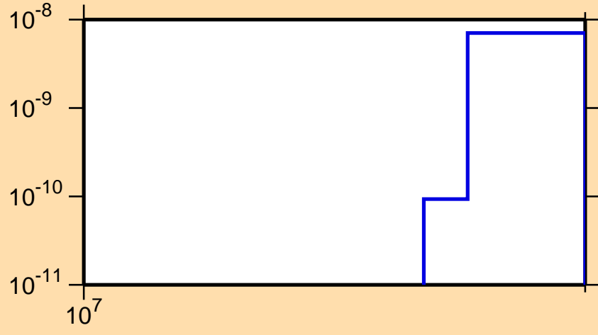
\sigma vs. E for ^{124}\text{Xe}(n,\text{pd})
