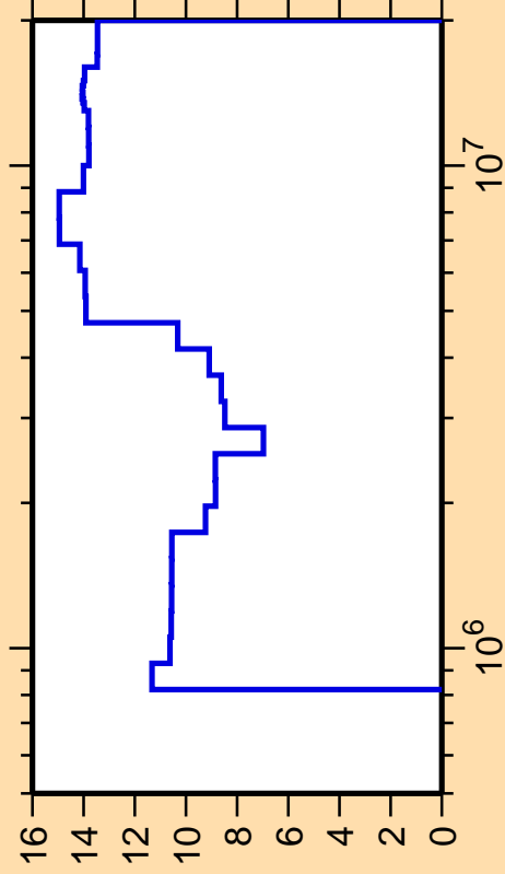
\Delta\sigma/\sigma vs. E for ^{124}\text{Xe}(n,n_2)
