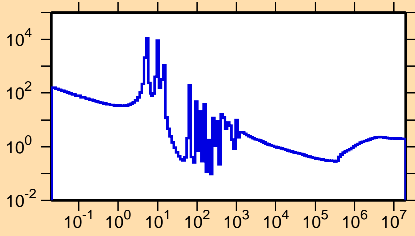
\sigma vs. E for ^{124}\text{Xe}(n,\text{nonel.})
