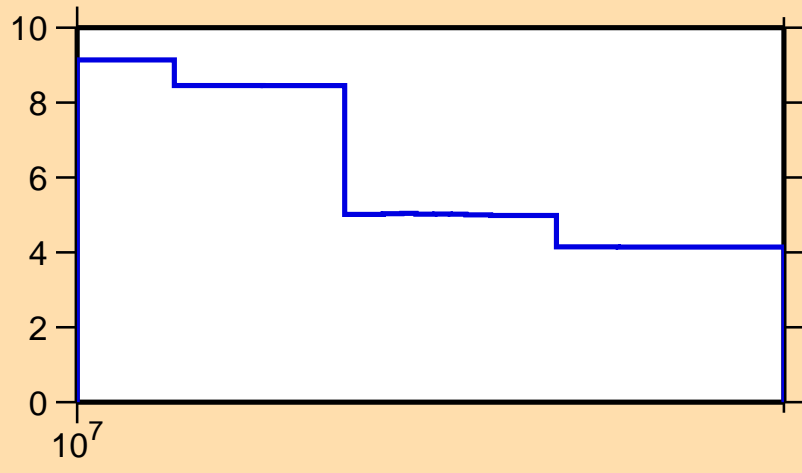
\Delta\sigma/\sigma vs. E for ^{124}\text{Xe}(n,2n)
