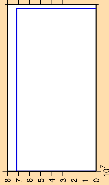
\Delta\sigma/\sigma vs. E for ^{124}\text{Xe}(n,n\text{cont.})
