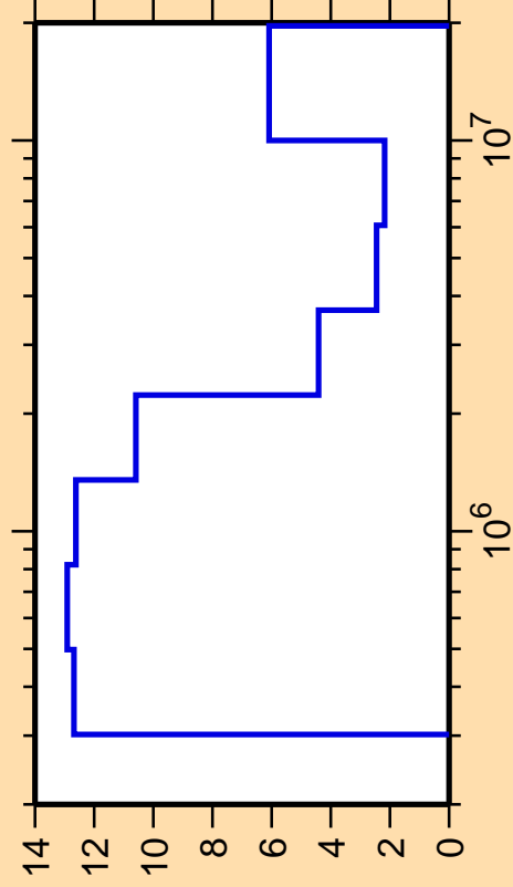
\Delta\sigma/\sigma vs. E for ^{124}\text{Xe}(n,\text{inel.})
