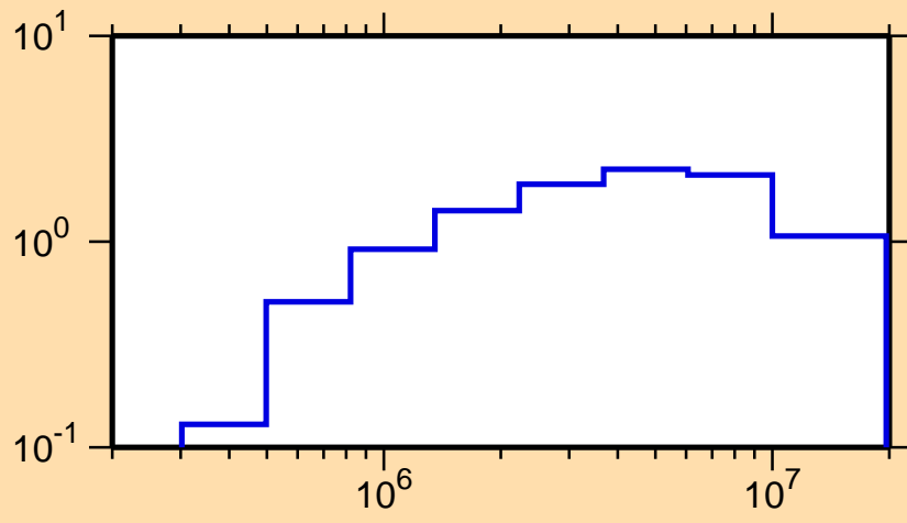
\sigma vs. E for ^{124}\text{Xe}(n,\text{inel.})
