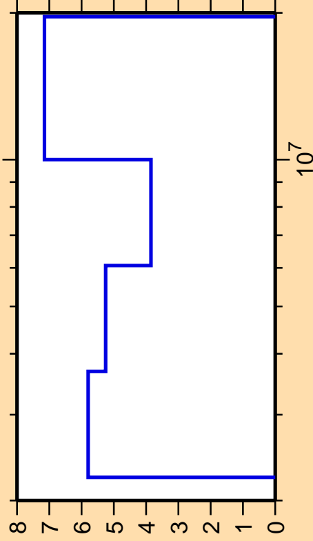
\Delta\sigma/\sigma vs. E for ^{124}\text{Xe}(n,n_{\text{cont}})
