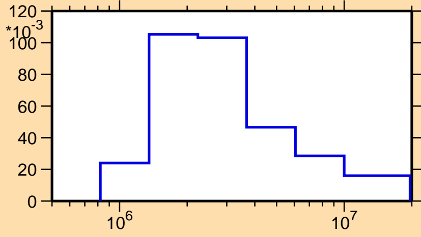
\sigma vs. E for ^{124}\text{Xe}(n,n_3)
