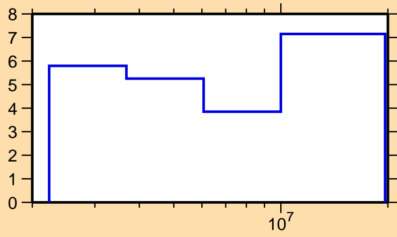
\Delta\sigma/\sigma vs. E for ^{124}\text{Xe}(n,n\text{cont.})
