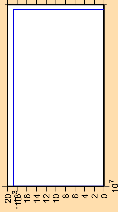
\Delta\sigma/\sigma vs. E for ^{124}\text{Xe}(\text{mt } 45)
