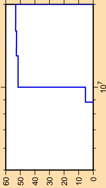
\Delta\sigma/\sigma vs. E for ^{125}\text{Xe}(n,p\alpha)
