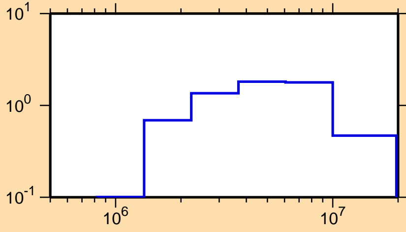
\sigma vs. E for ^{125}\text{Xe}(n,n\text{cont.})
