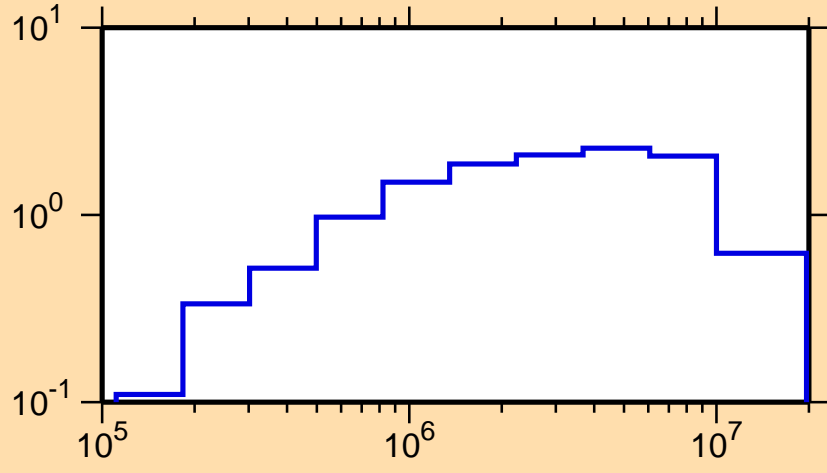
\sigma vs. E for ^{125}\text{Xe}(n,\text{inel.})
