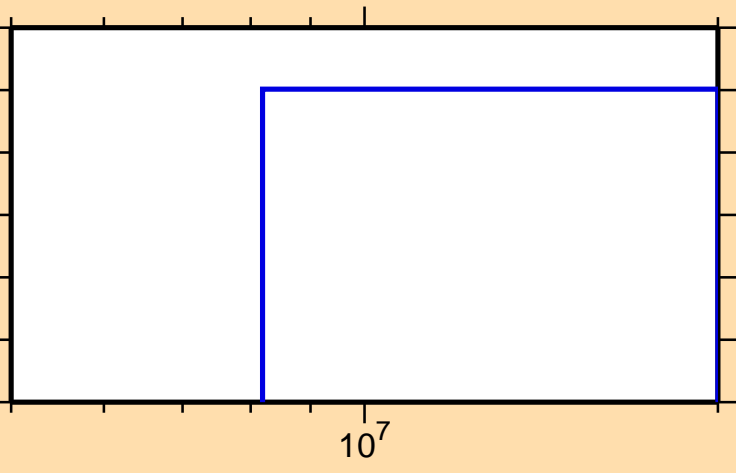
\sigma vs. E for ^{125}\text{Xe}(n,\text{He}3)
