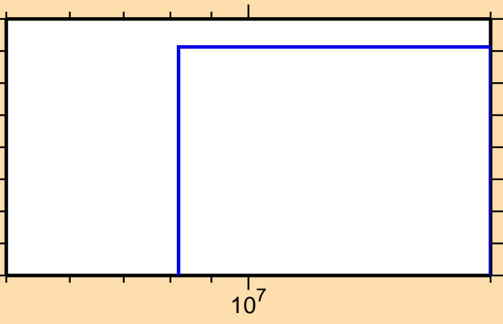
\sigma vs. E for ^{125}\text{Xe}(n,p\alpha)
