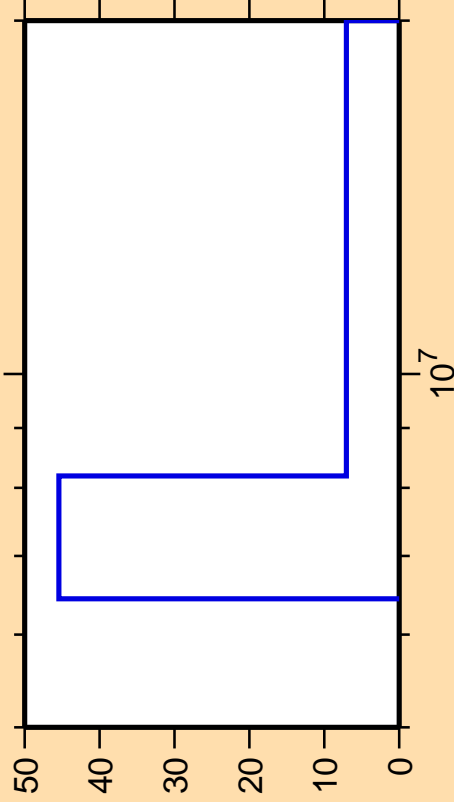
\Delta\sigma/\sigma vs. E for ^{125}\text{Xe}(n,2n)
