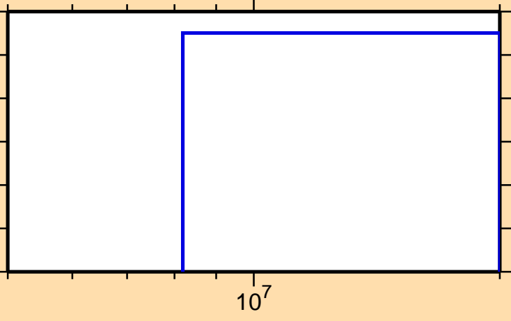
\sigma vs. E for ^{125}\text{Xe}(n,\text{nd})
