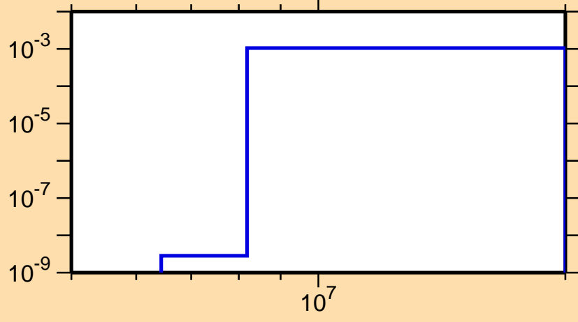
\sigma vs. E for ^{125}\text{Xe}(n,n\alpha)
