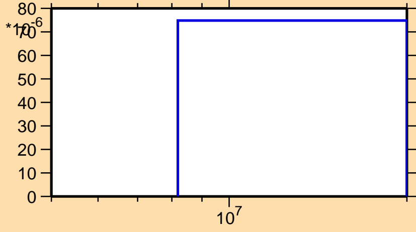
\sigma vs. E for ^{125}\text{Xe}(n,t)
