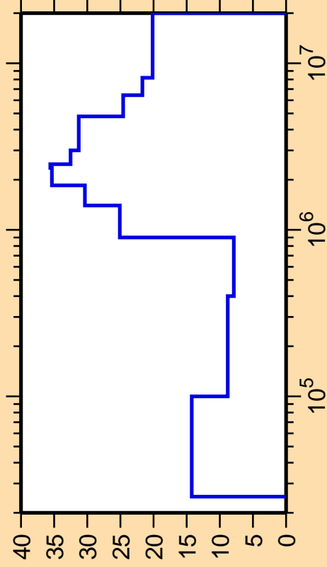
\Delta\sigma/\sigma vs. E for ^{125}\text{Xe}(n,n_4)
