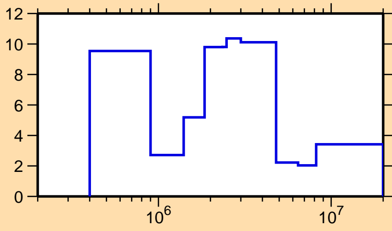
\Delta\sigma/\sigma vs. E for ^{125}\text{Xe}(n, el.)
