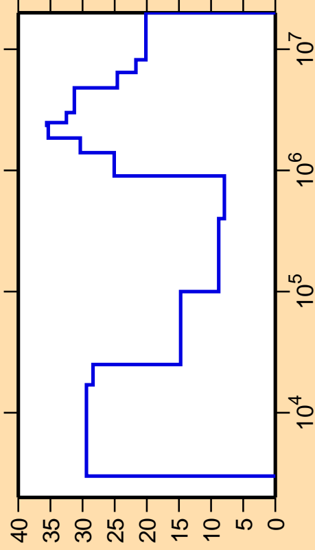
\Delta\sigma/\sigma vs. E for ^{125}\text{Xe}(n,n_3)
