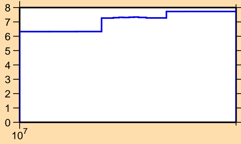
\Delta\sigma/\sigma vs. E for ^{126}\text{Xe}(n,\text{inel.})
