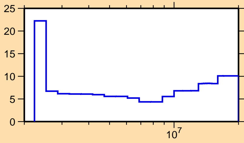
\Delta\sigma/\sigma vs. E for ^{126}\text{Xe}(n,n\text{cont.})
