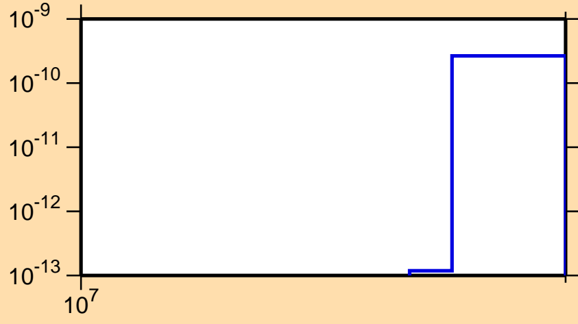
\sigma vs. E for ^{126}\text{Xe}(n,2n\alpha)
