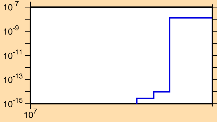
\sigma vs. E for ^{126}\text{Xe}(n,nd)
