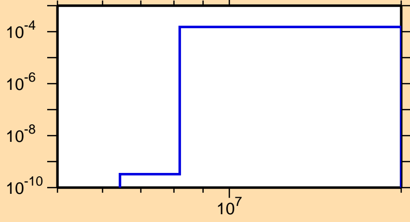
\sigma vs. E for ^{126}\text{Xe}(n,n\alpha)
