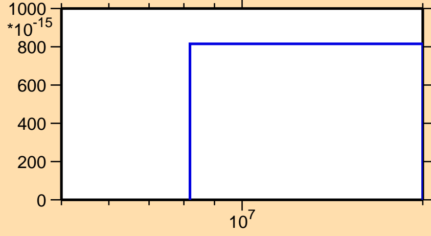
\sigma vs. E for ^{126}\text{Xe}(n,\text{pd})
