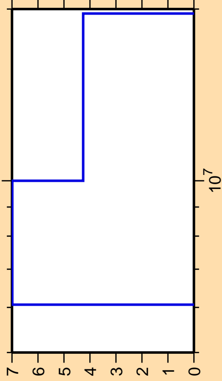
\Delta\sigma/\sigma vs. E for ^{127}\text{Xe}(n,2n)
