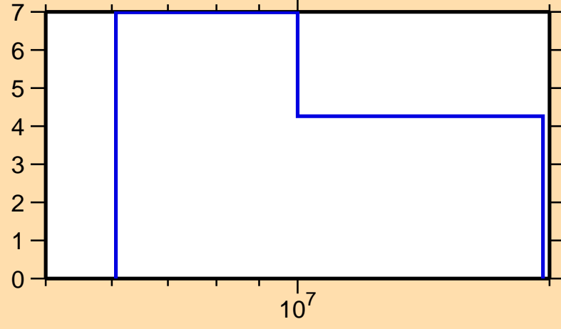
\Delta\sigma/\sigma vs. E for ^{127}\text{Xe}(n,2n)
