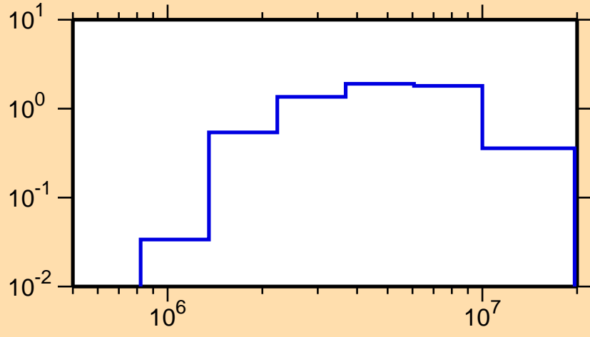
\sigma vs. E for ^{127}\text{Xe}(n,n\text{cont.})
