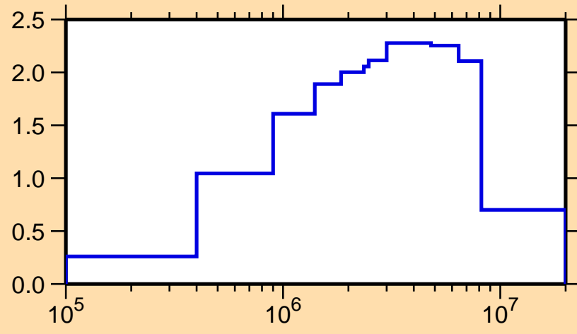
\sigma vs. E for ^{127}\text{Xe}(n,\text{inel.})
