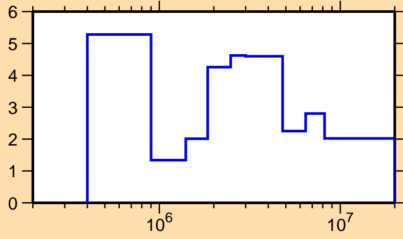
\Delta\sigma/\sigma vs. E for ^{127}\text{Xe}(n,\text{el.})
