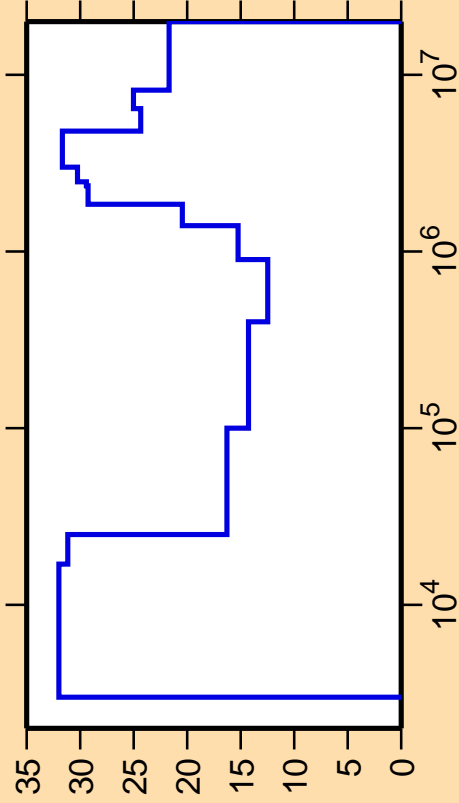
\Delta\sigma/\sigma vs. E for ^{127}\text{Xe}(n,n_3)
