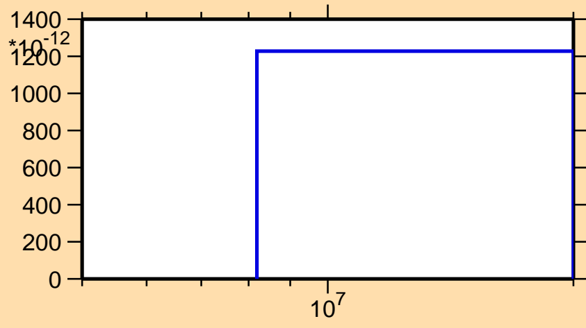
\sigma vs. E for ^{127}\text{Xe}(n,\text{He}3)
