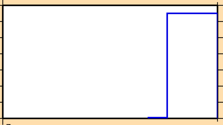
\sigma vs. E for ^{128}\text{Xe}(n,3n)
