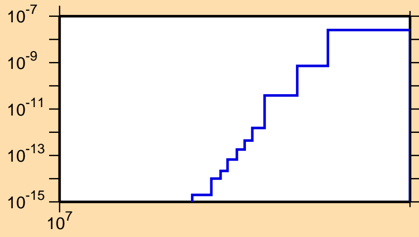
\sigma vs. E for ^{128}\text{Xe}(n,\text{He}3)
