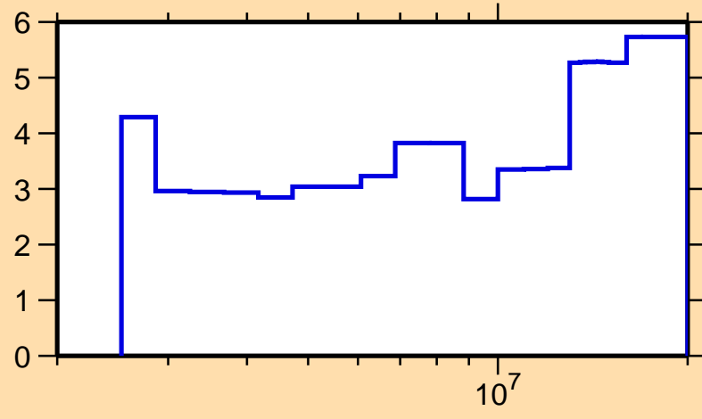
\Delta\sigma/\sigma vs. E for ^{128}\text{Xe}(n,\text{inel.})
