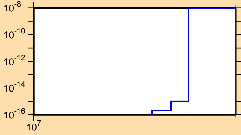
\sigma vs. E for ^{128}\text{Xe}(n,nd)
