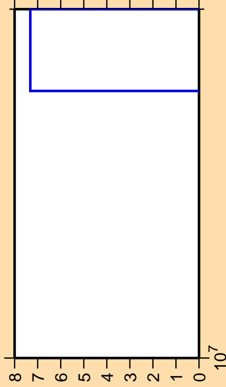
\Delta\sigma/\sigma vs. E for ^{128}\text{Xe}(n,2np)
