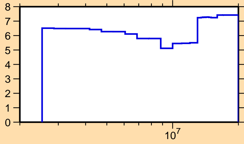
\Delta\sigma/\sigma vs. E for ^{128}\text{Xe}(n,n\text{cont.})
