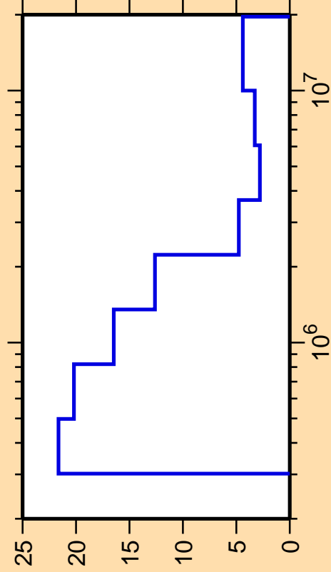
\Delta\sigma/\sigma vs. E for ^{128}\text{Xe}(n,\text{inel.})
