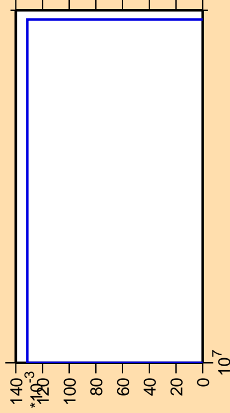
\Delta\sigma/\sigma vs. E for ^{128}\text{Xe}(n,nt)
