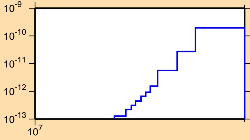
\sigma vs. E for ^{129}\text{Xe}(n,p\alpha)
