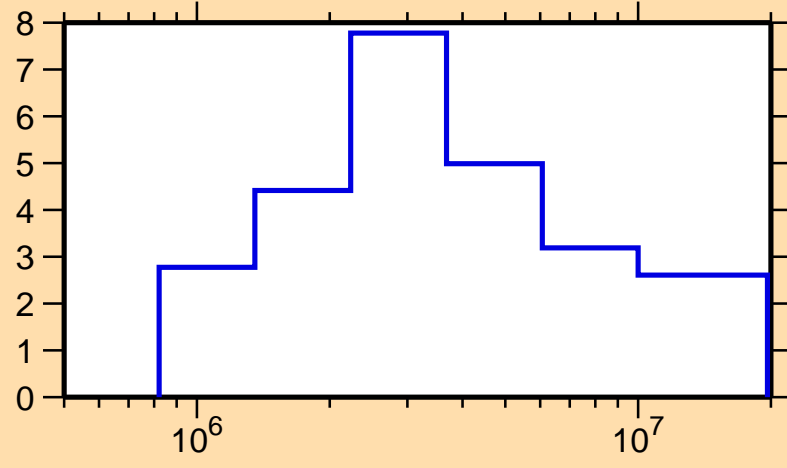
\Delta\sigma/\sigma vs. E for ^{129}\text{Xe}(n, el.)
