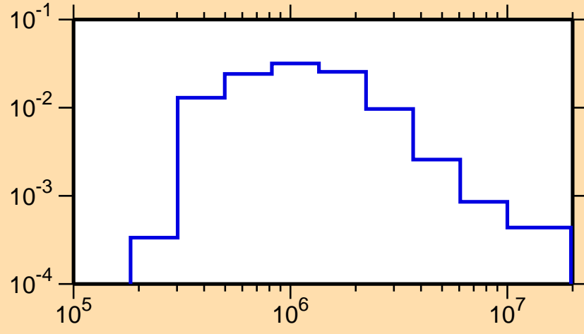
\sigma vs. E for ^{129}\text{Xe}(n,n_3)
