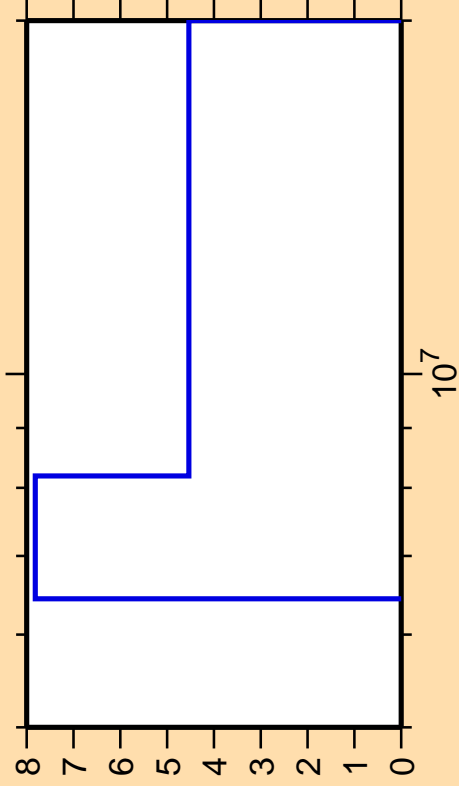
\Delta\sigma/\sigma vs. E for ^{129}\text{Xe}(n,2n)
