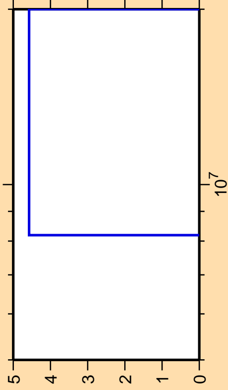
\Delta\sigma/\sigma vs. E for ^{129}\text{Xe}(n,p\alpha)
