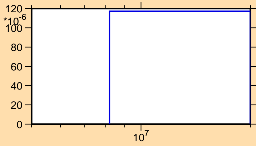
\sigma vs. E for ^{129}\text{Xe}(n,t)
