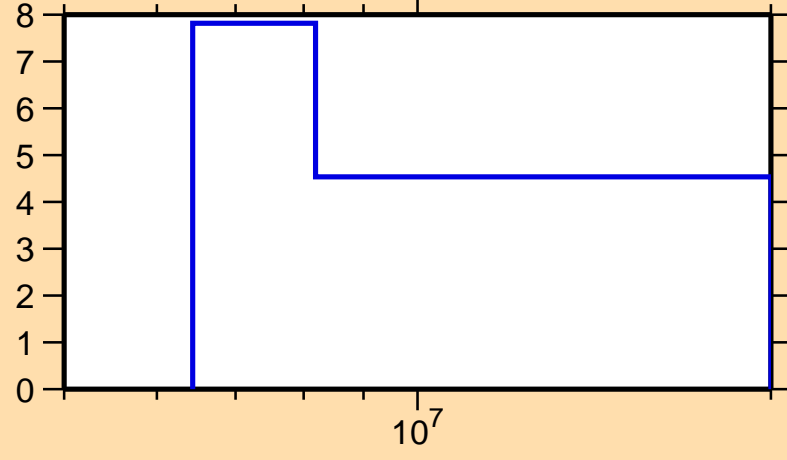
\Delta\sigma/\sigma vs. E for ^{129}\text{Xe}(n,2n)
