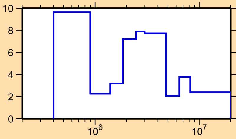
\Delta\sigma/\sigma vs. E for ^{129}\text{Xe}(n,el.)
