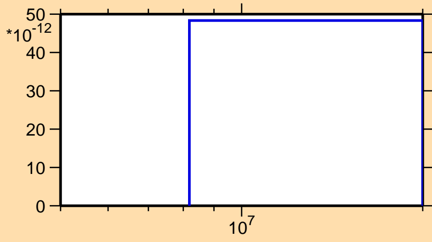
\sigma vs. E for ^{129}\text{Xe}(n,\text{He}3)
