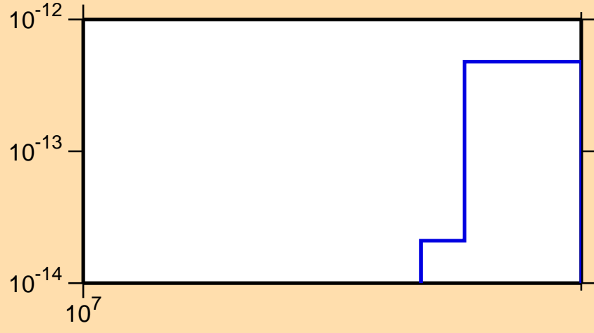
\sigma vs. E for ^{130}\text{Xe}(n,p\alpha)
