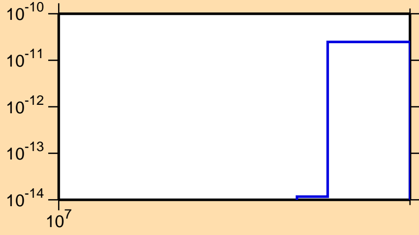
\sigma vs. E for ^{130}\text{Xe}(n,2n\alpha)
